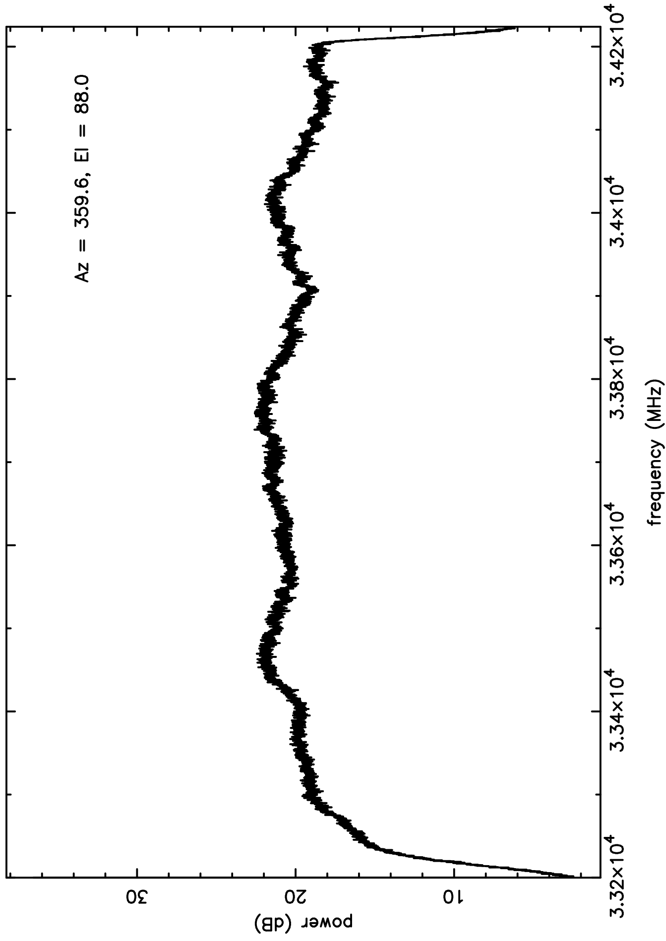
Ka-band RFI plot (mean power) - IF D - ea24
