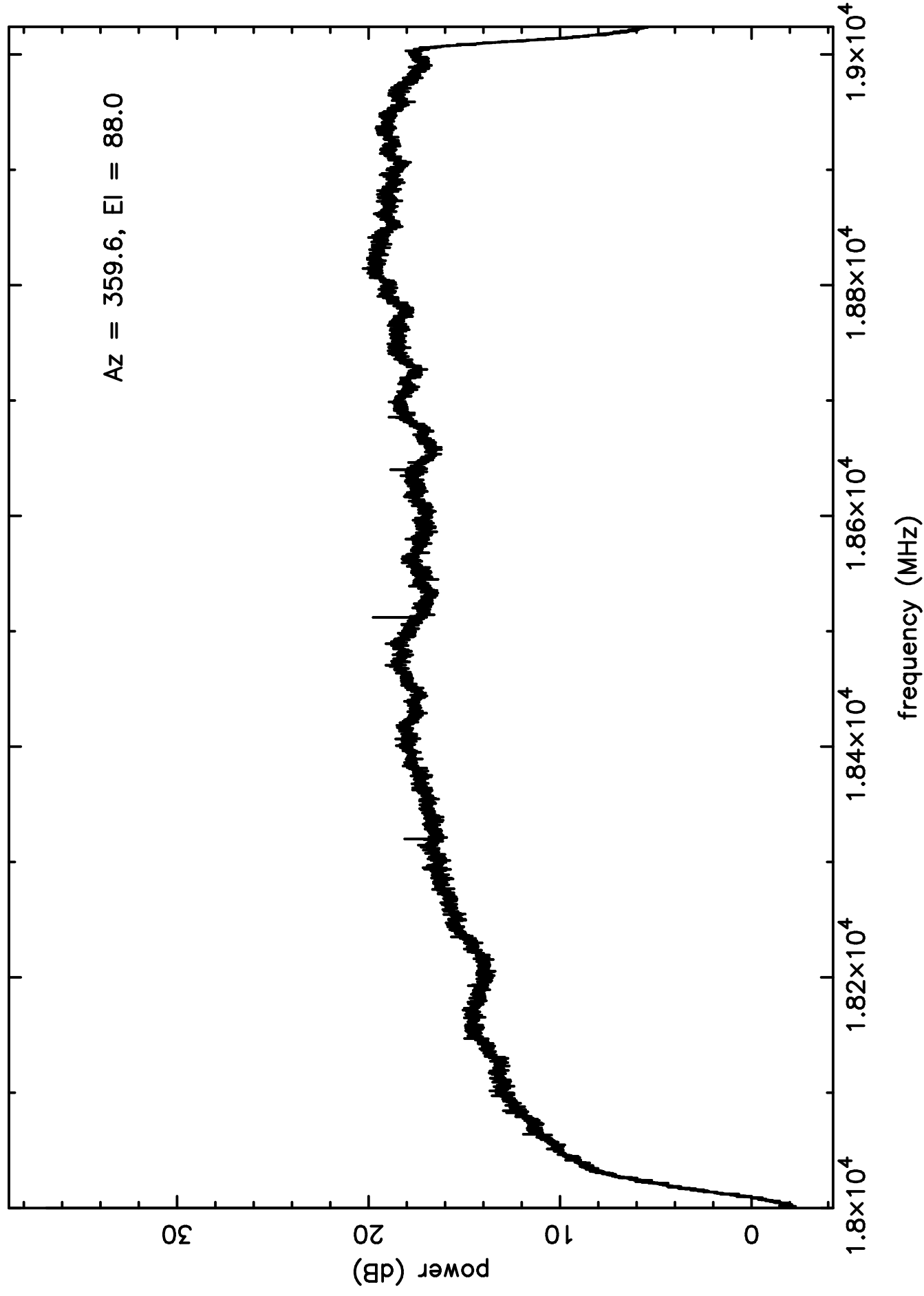
K-band RFI plot (mean power) - IF D - ea24
