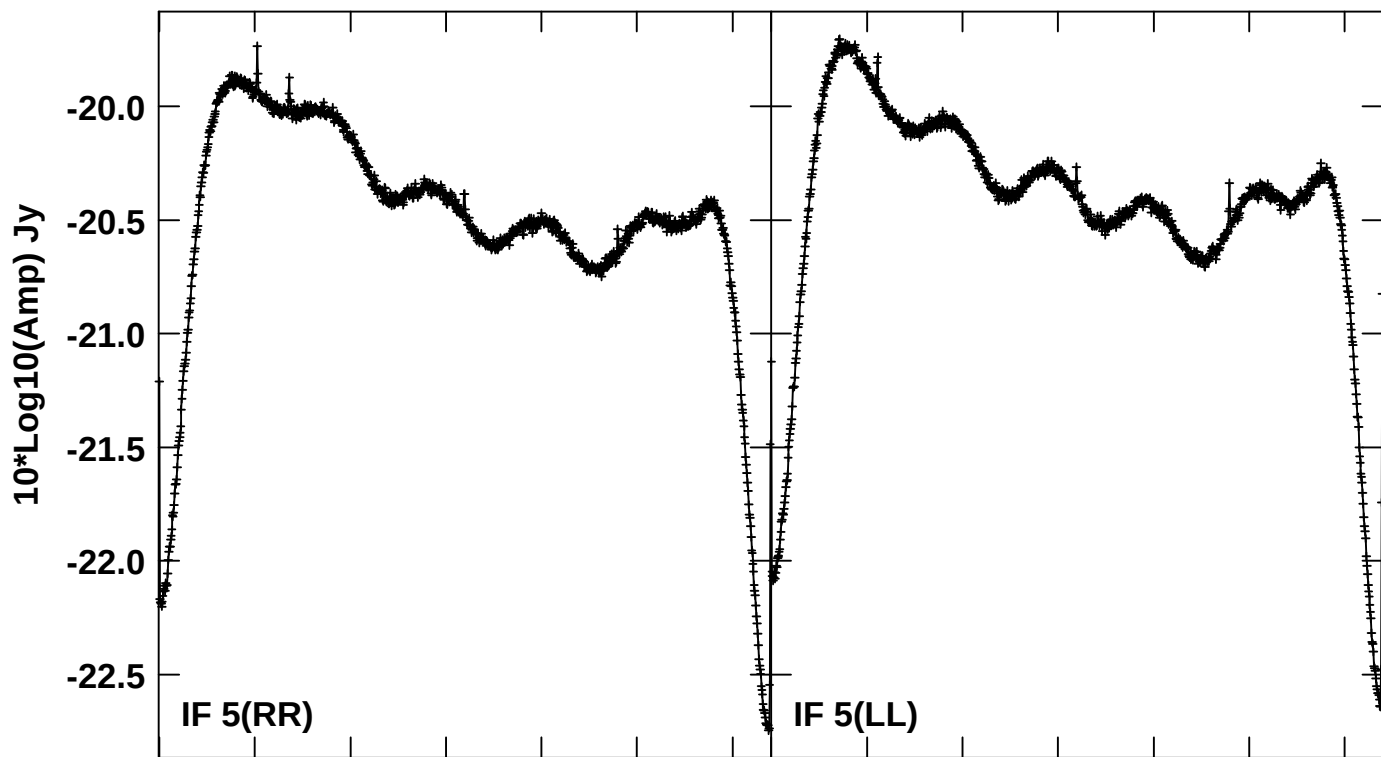
25500 25520 25540 25560 25580 25600 25620 FREQ MHz Scalar averaged cross-power spectrum Several baselines averaged
