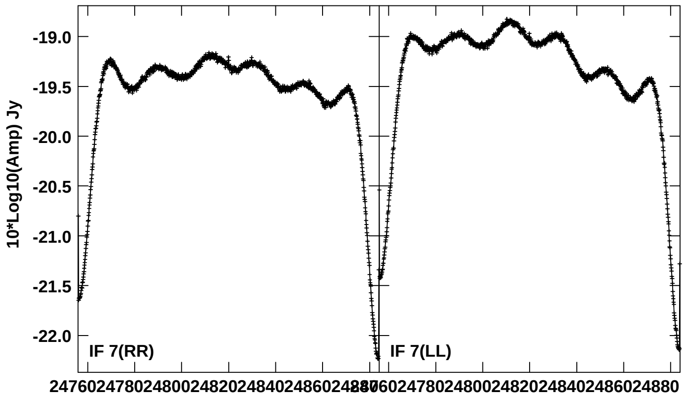
Scalar averaged cross-power spectrum Several baselines averaged
