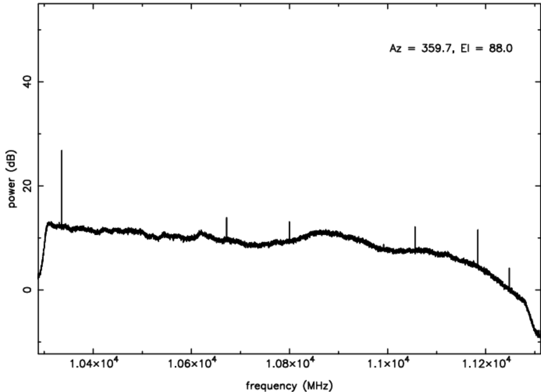
X-band RFI plot (mean power) – IF D – ea12
