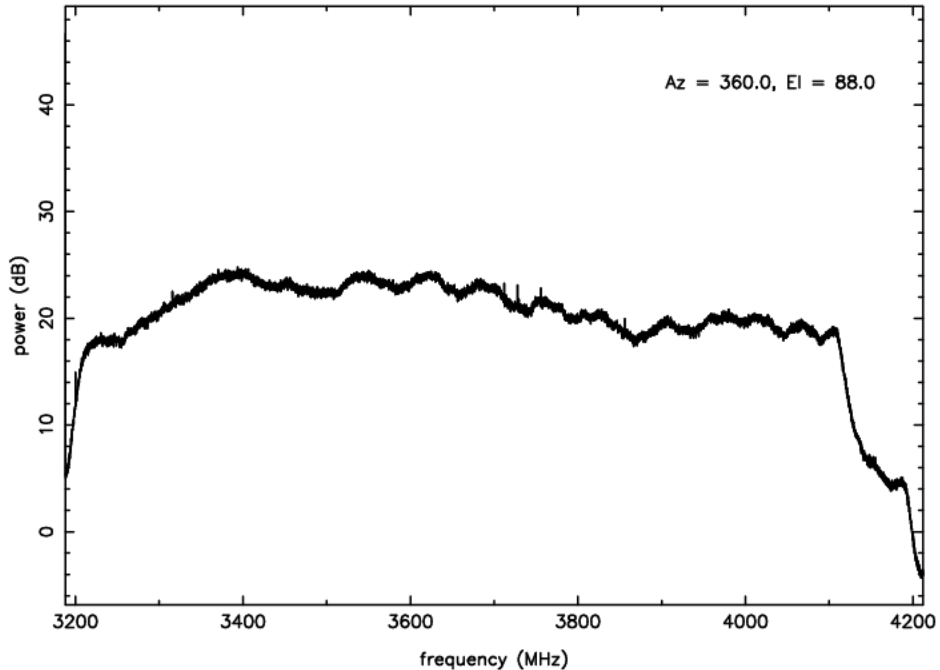
S-band RFI plot (mean power) – IF B – ea12
