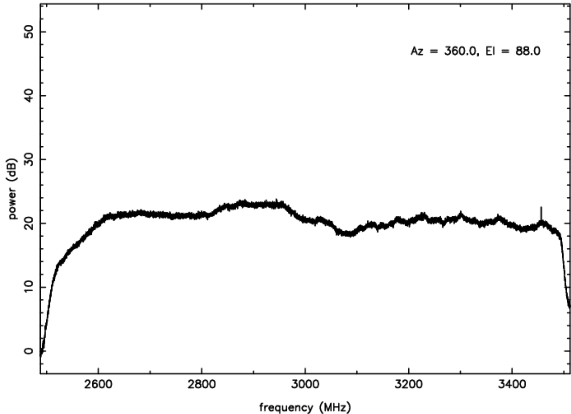
S-band RFI plot (mean power) – IF D – ea12
