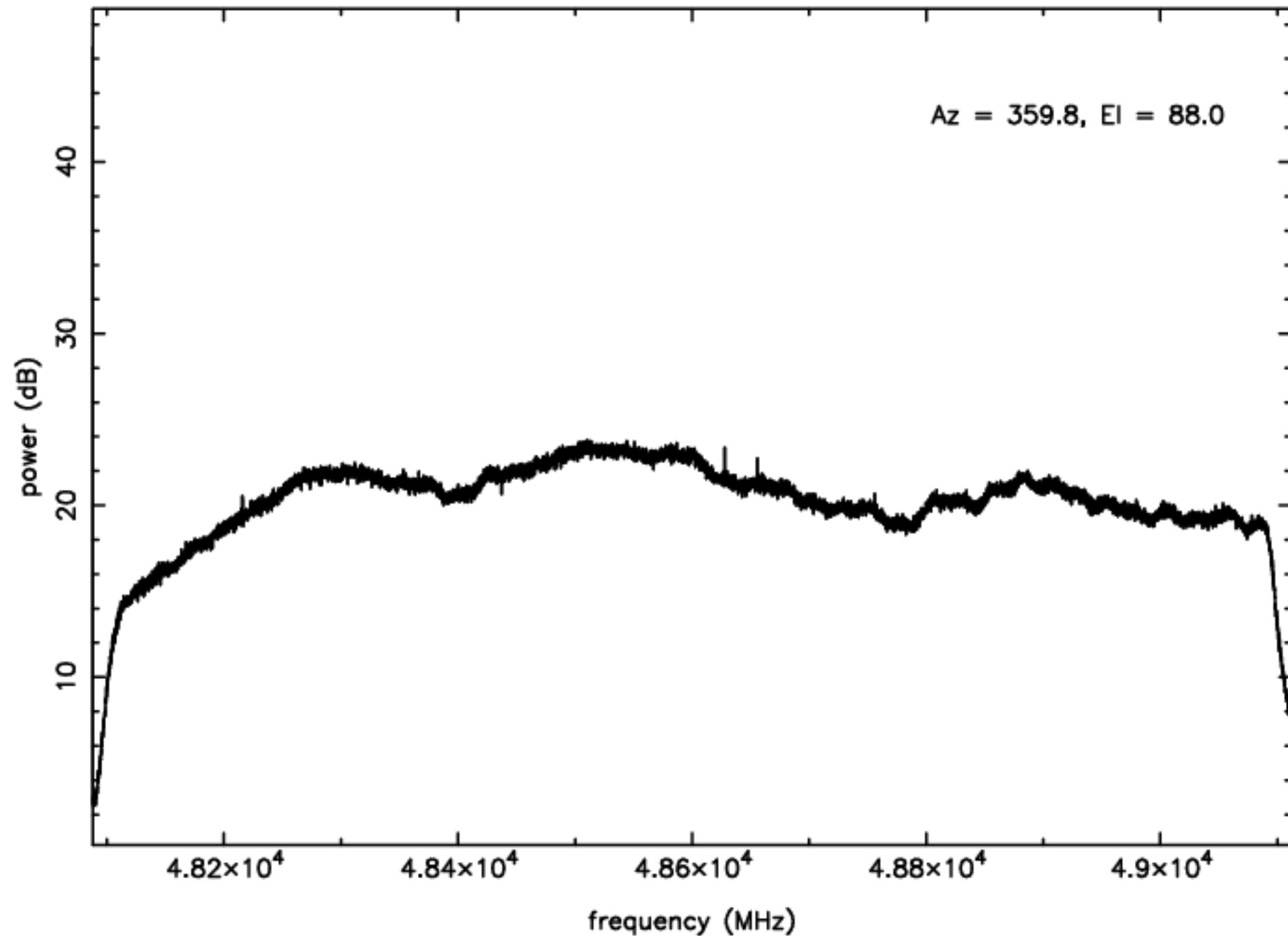
Q-band RFI plot (mean power) - IF B - ea12
