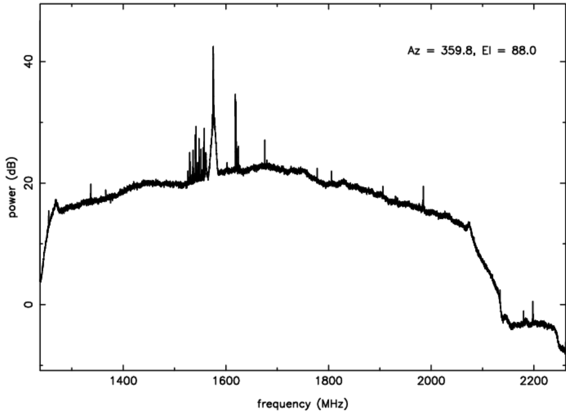
L-band RFI plot (mean power) – IF B – ea12
