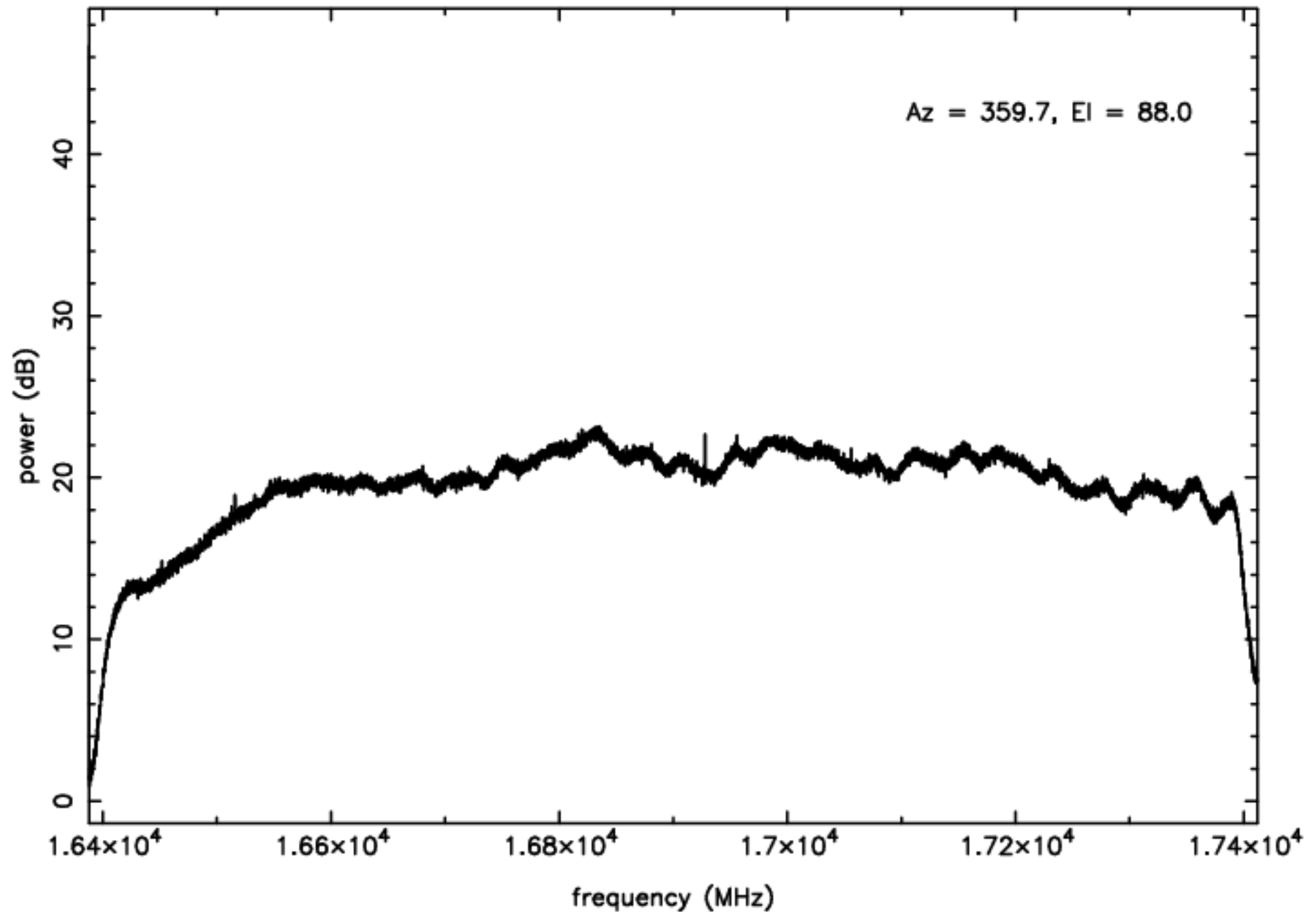
Ku-band RFI plot (mean power) - IF B - ea12
