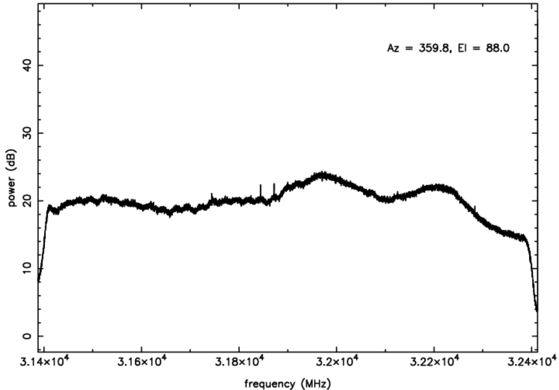
Ka-band RFI plot (mean power) - IF B - ea12
