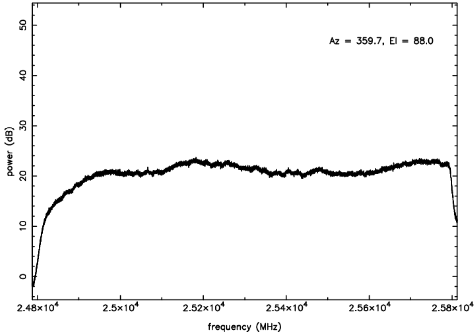
K-band RFI plot (mean power) – IF D – ea12
