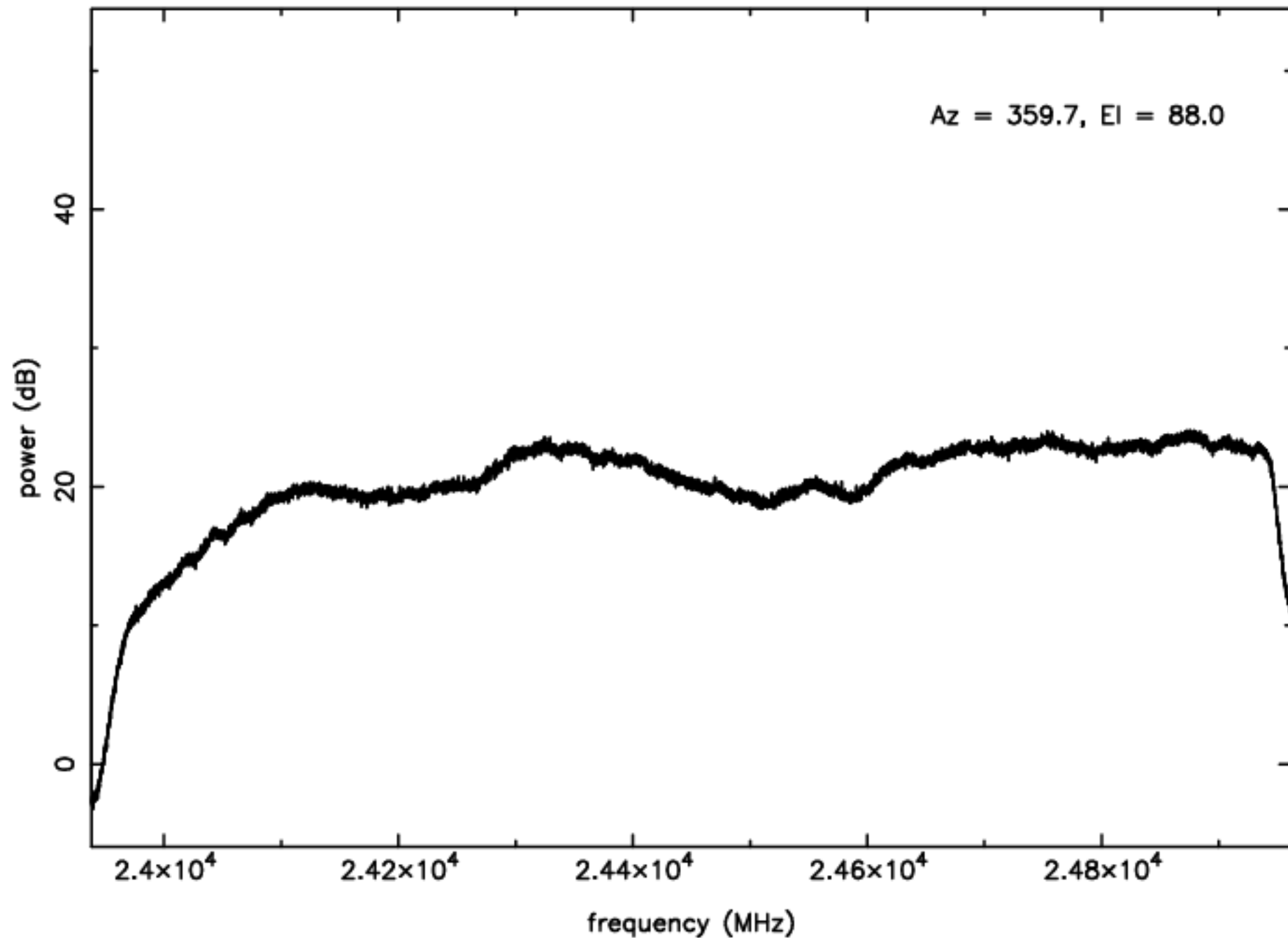
K-band RFI plot (mean power) – IF D – ea12
