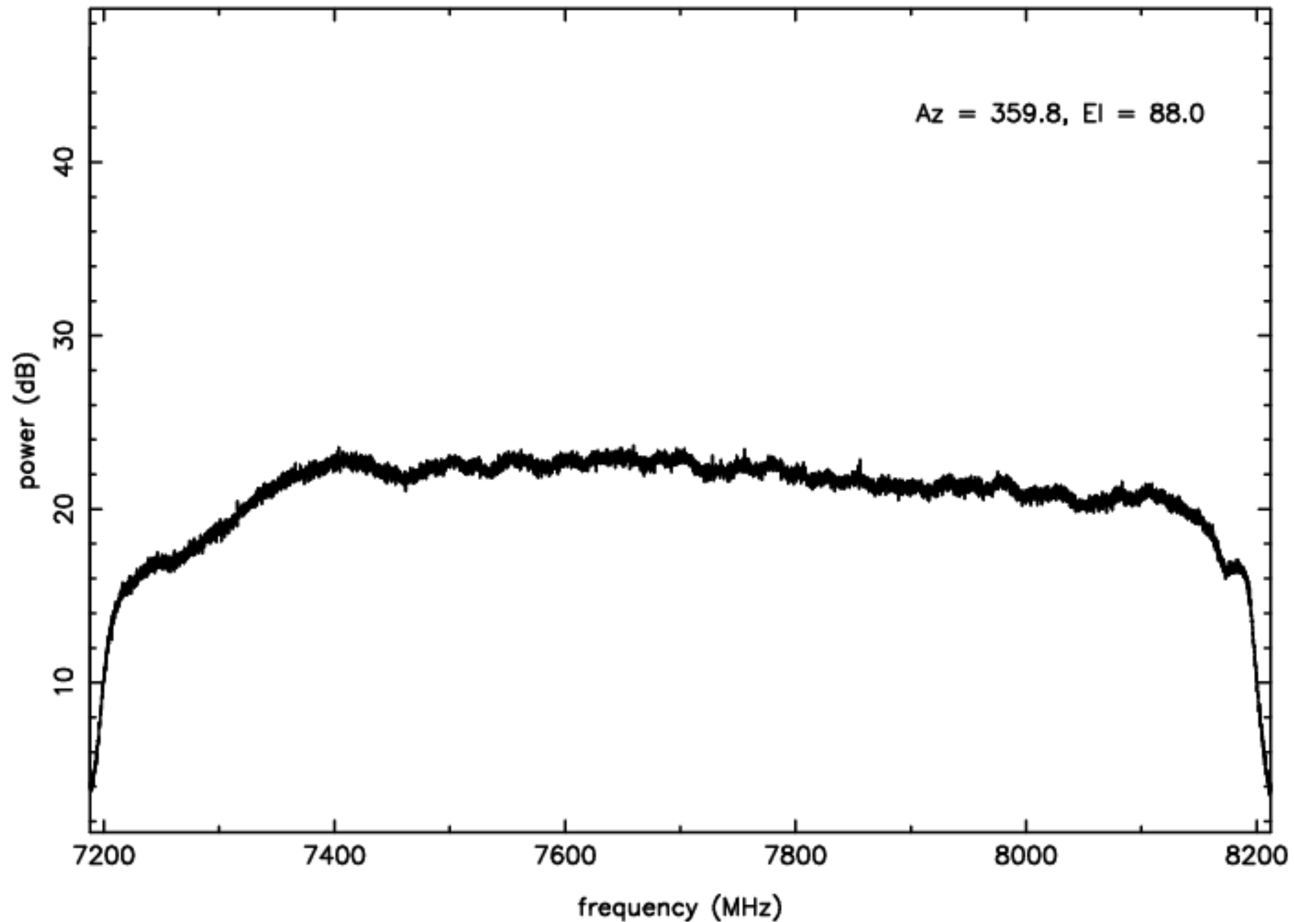
C-band RFI plot (mean power) – IF B – ea12
