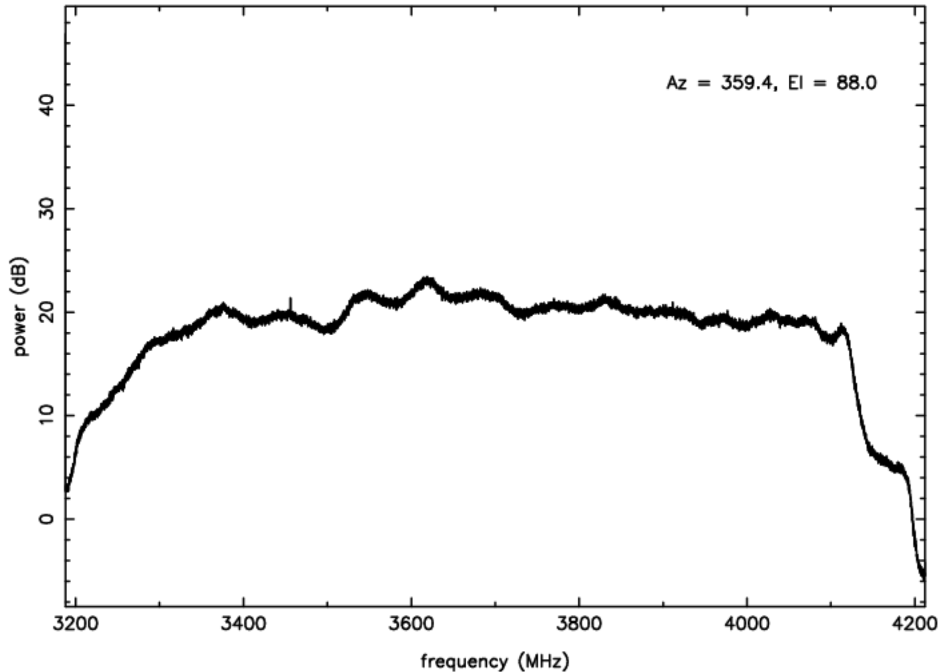
S-band RFI plot (mean power) – IF D – ea10
