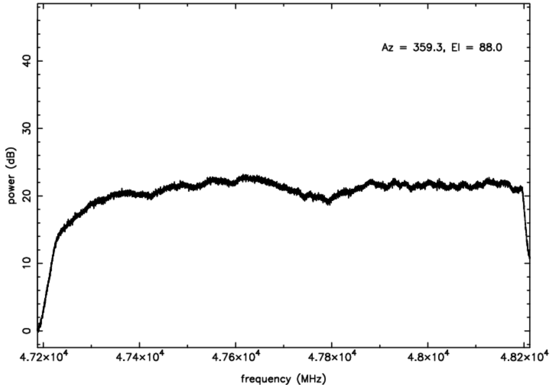
Q-band RFI plot (mean power) – IF B – ea10
