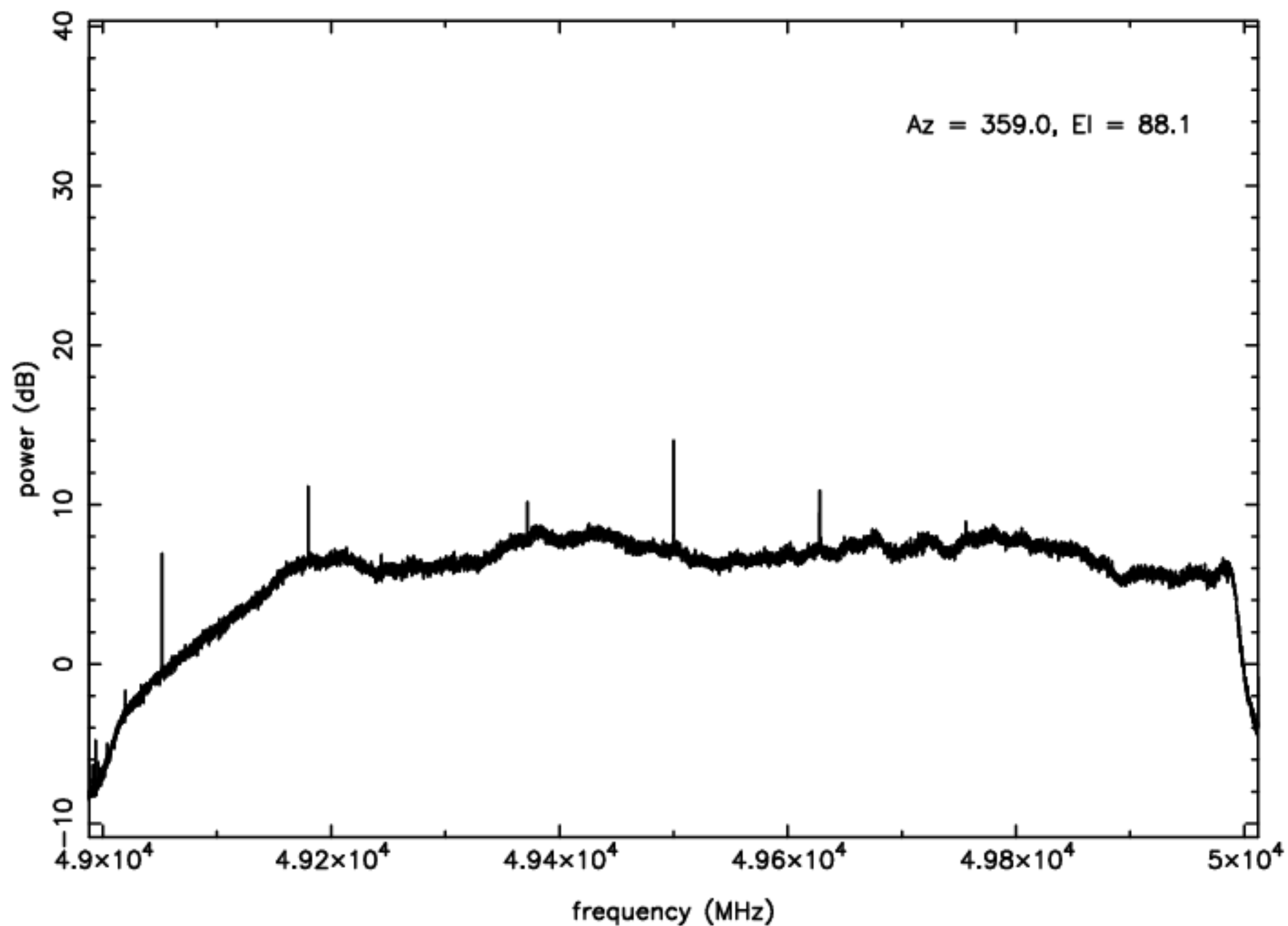
Q-band RFI plot (mean power) – IF D – ea22
