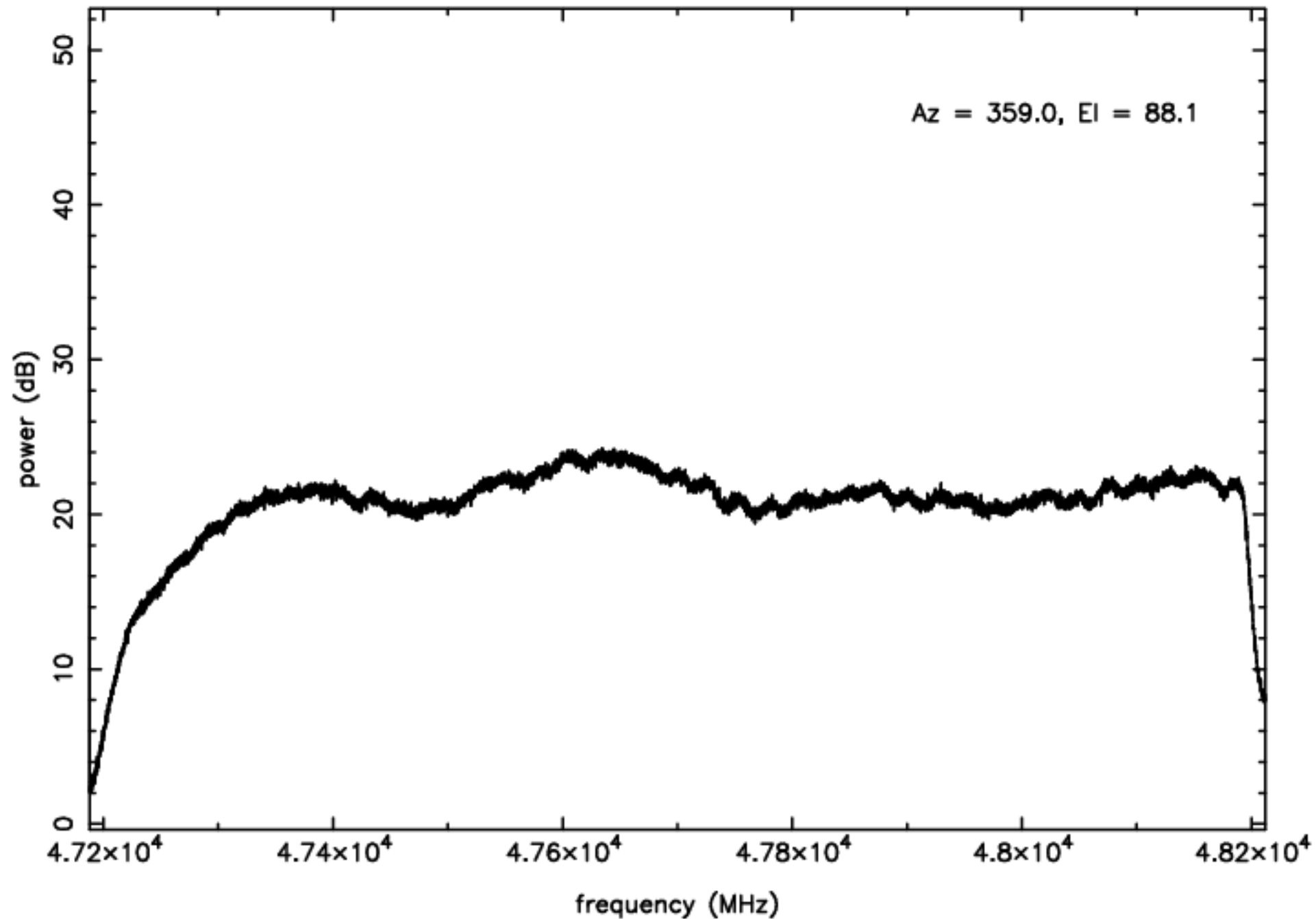
Q-band RFI plot (mean power) – IF B – ea22
