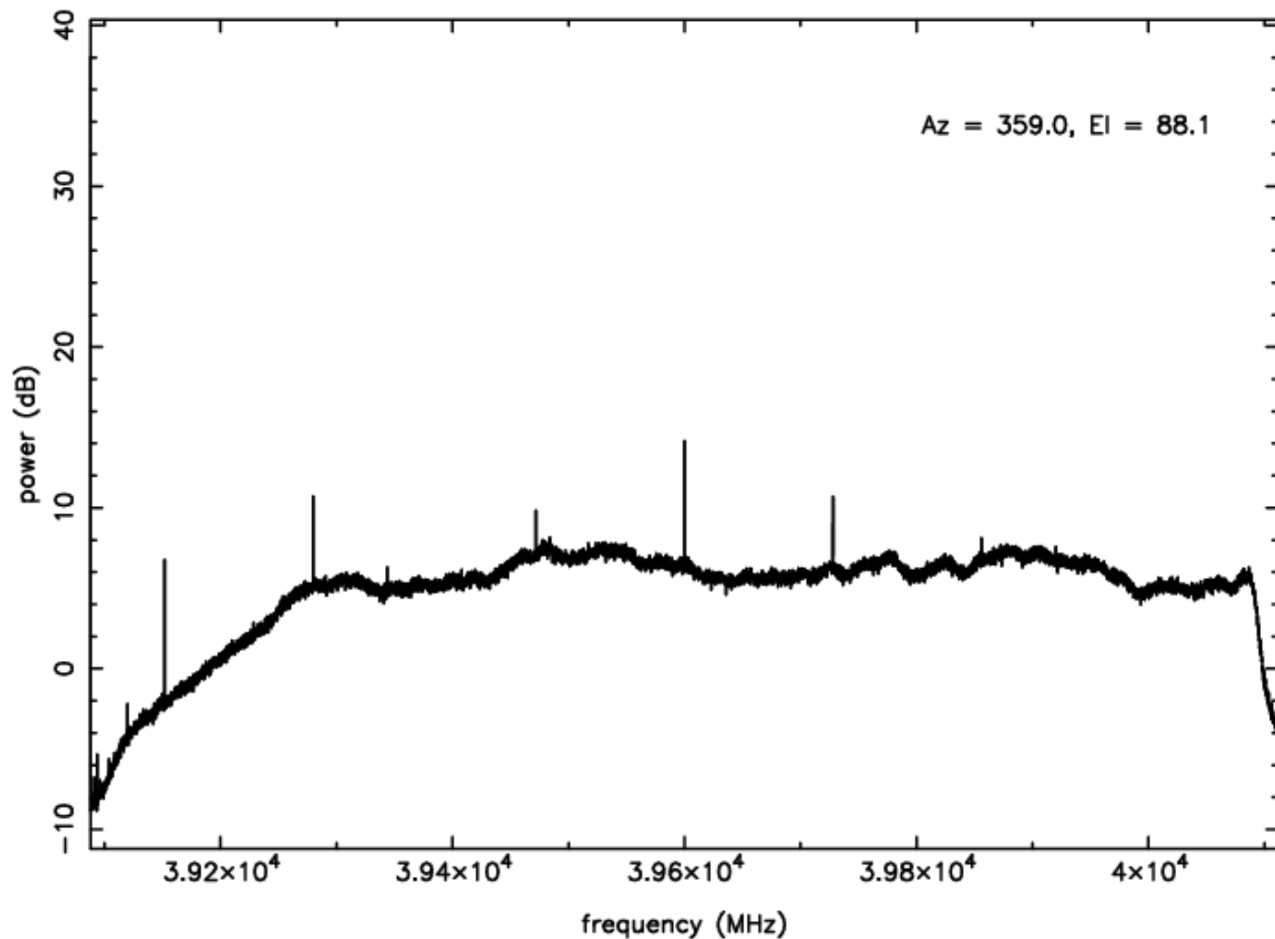
Q-band RFI plot (mean power) – IF D – ea22
