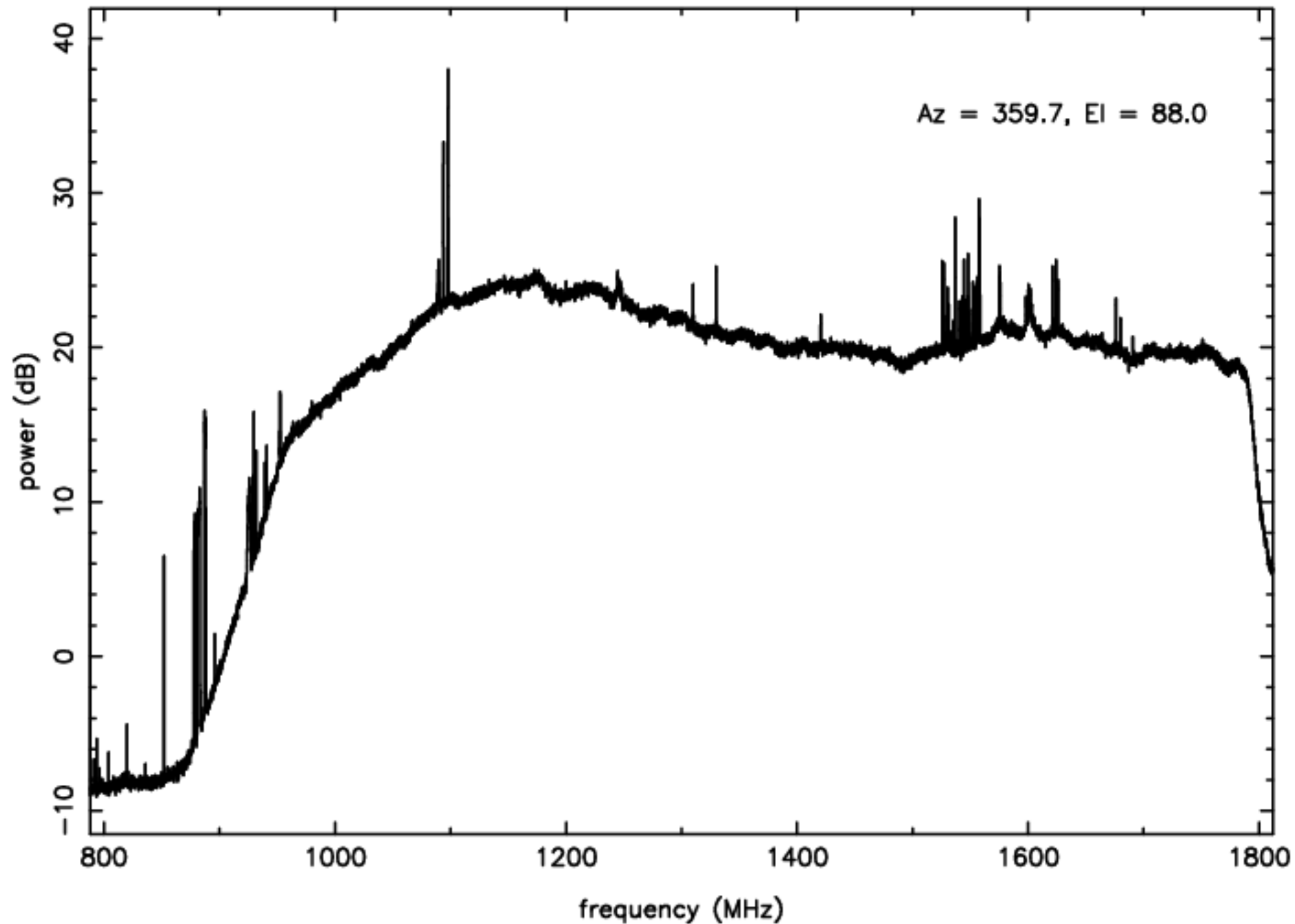
L-band RFI plot (mean power) – IF D – ea22
