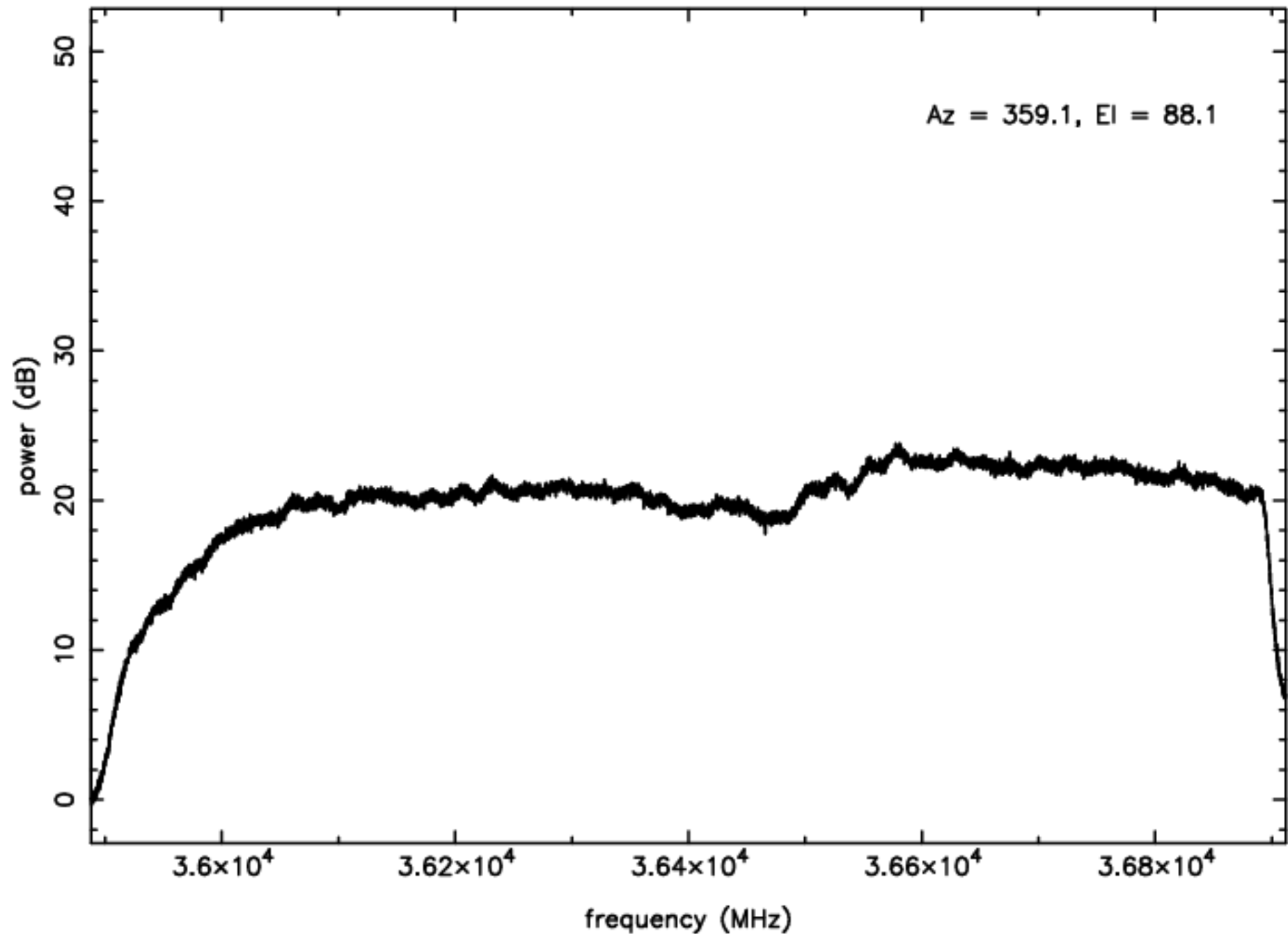
Ka-band RFI plot (mean power) – IF B – ea22
