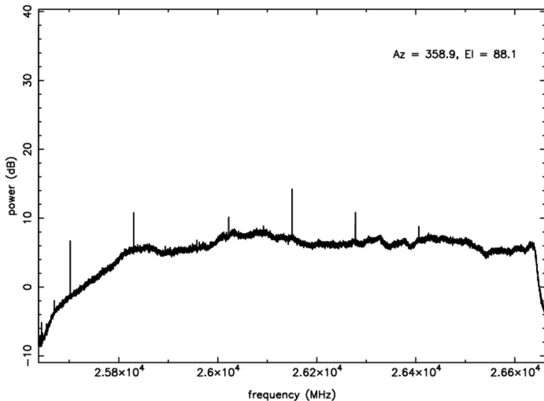
K-band RFI plot (mean power) – IF D – ea22
