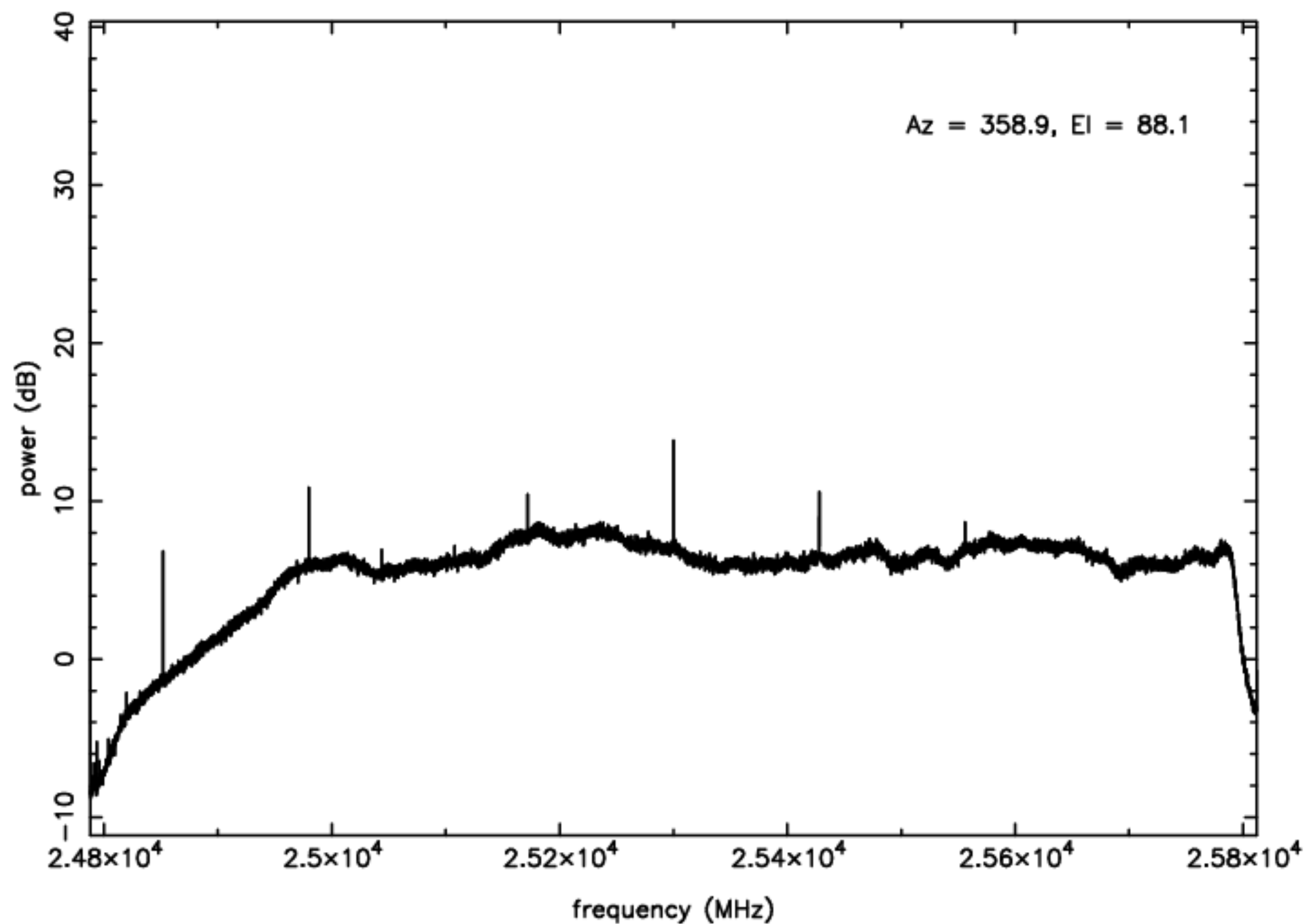
K-band RFI plot (mean power) – IF D – ea22
