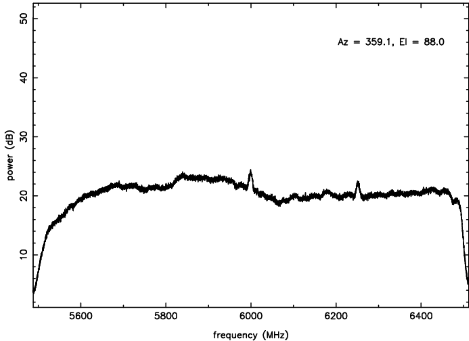
C-band RFI plot (mean power) – IF B – ea22
