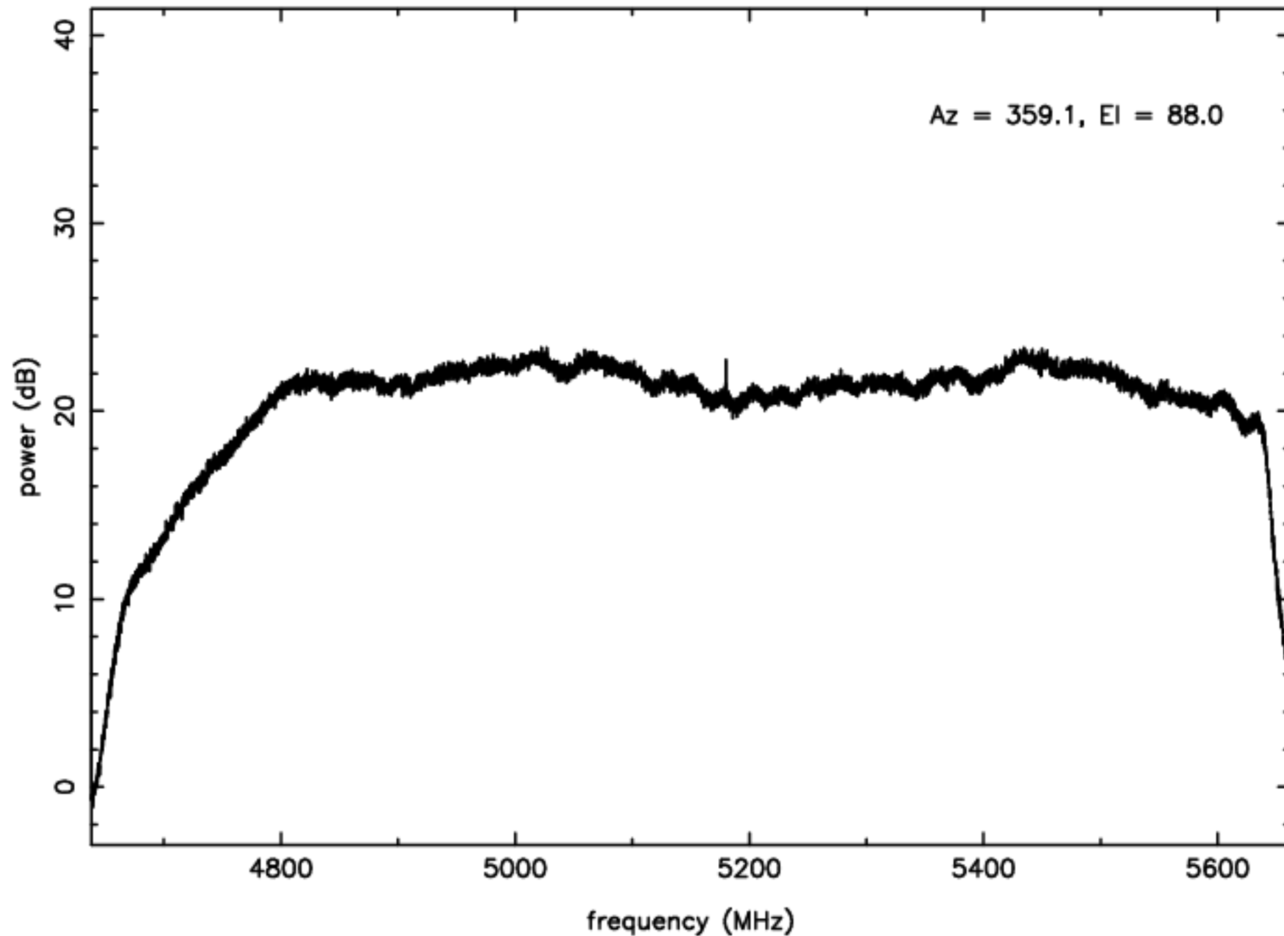
C-band RFI plot (mean power) – IF D – ea22
