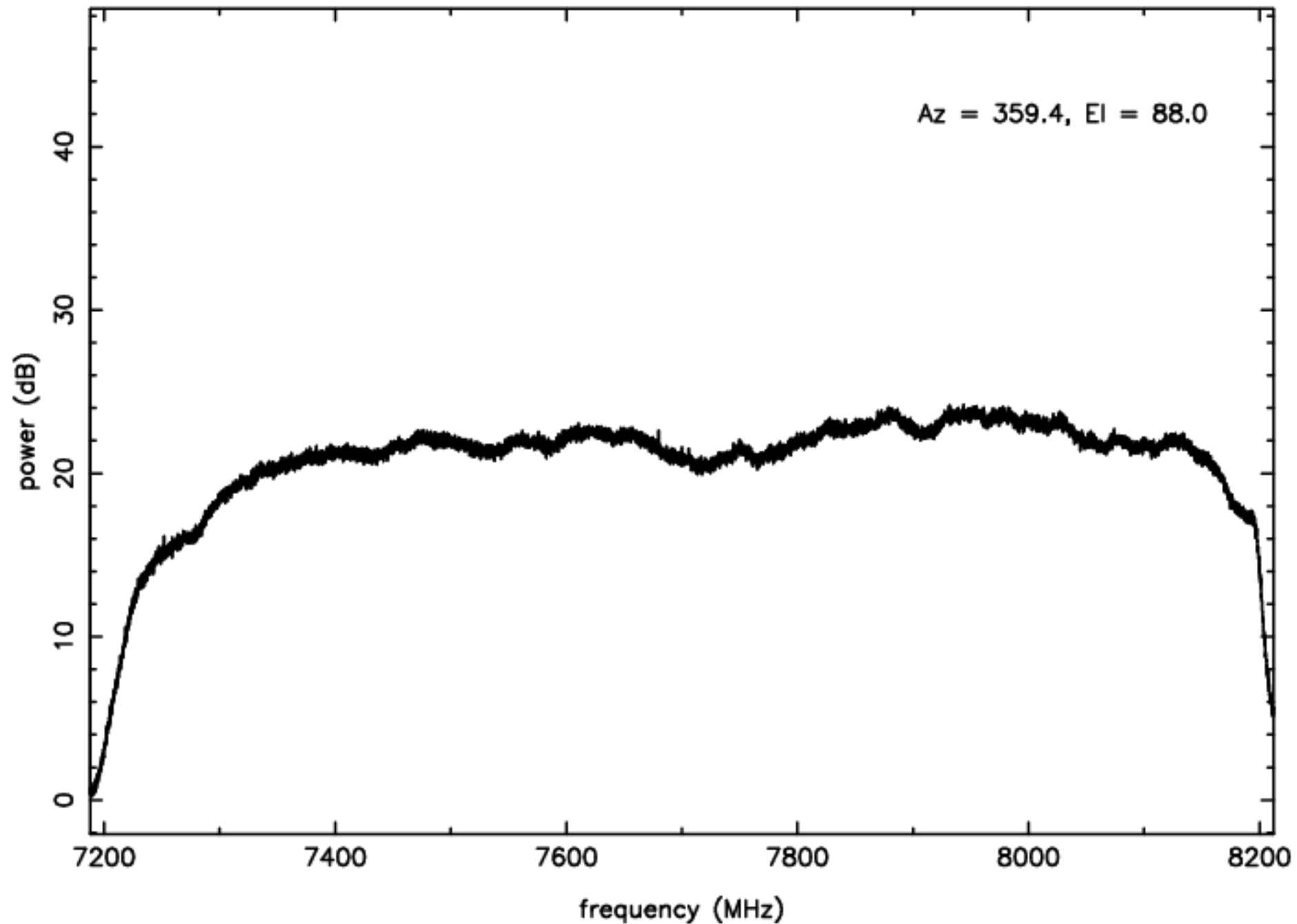
C-band RFI plot (mean power) – IF B – ea10
