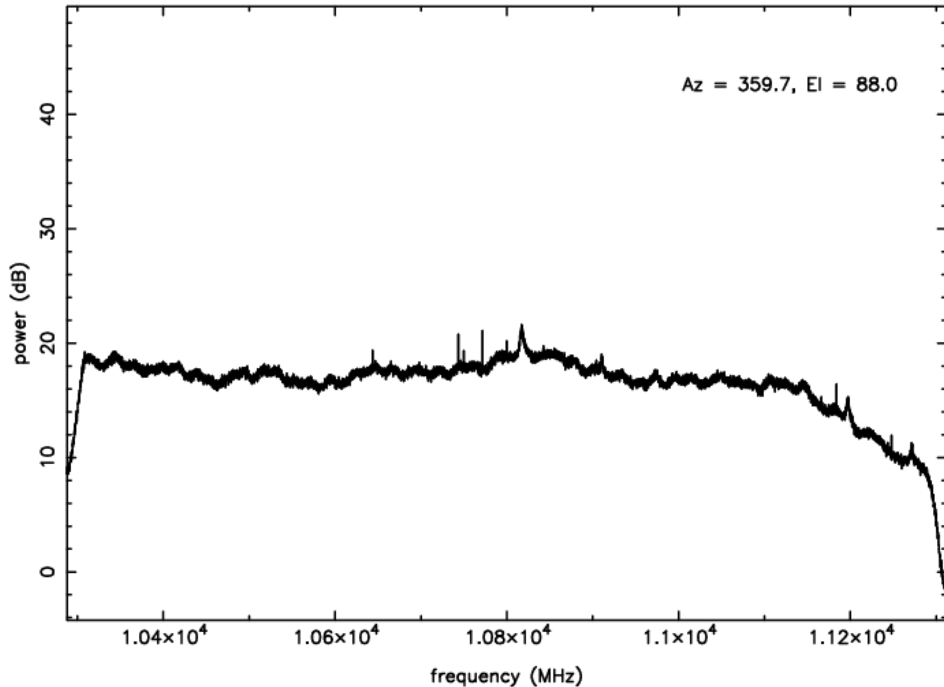
X-band RFI plot (mean power) – IF B – ea12
