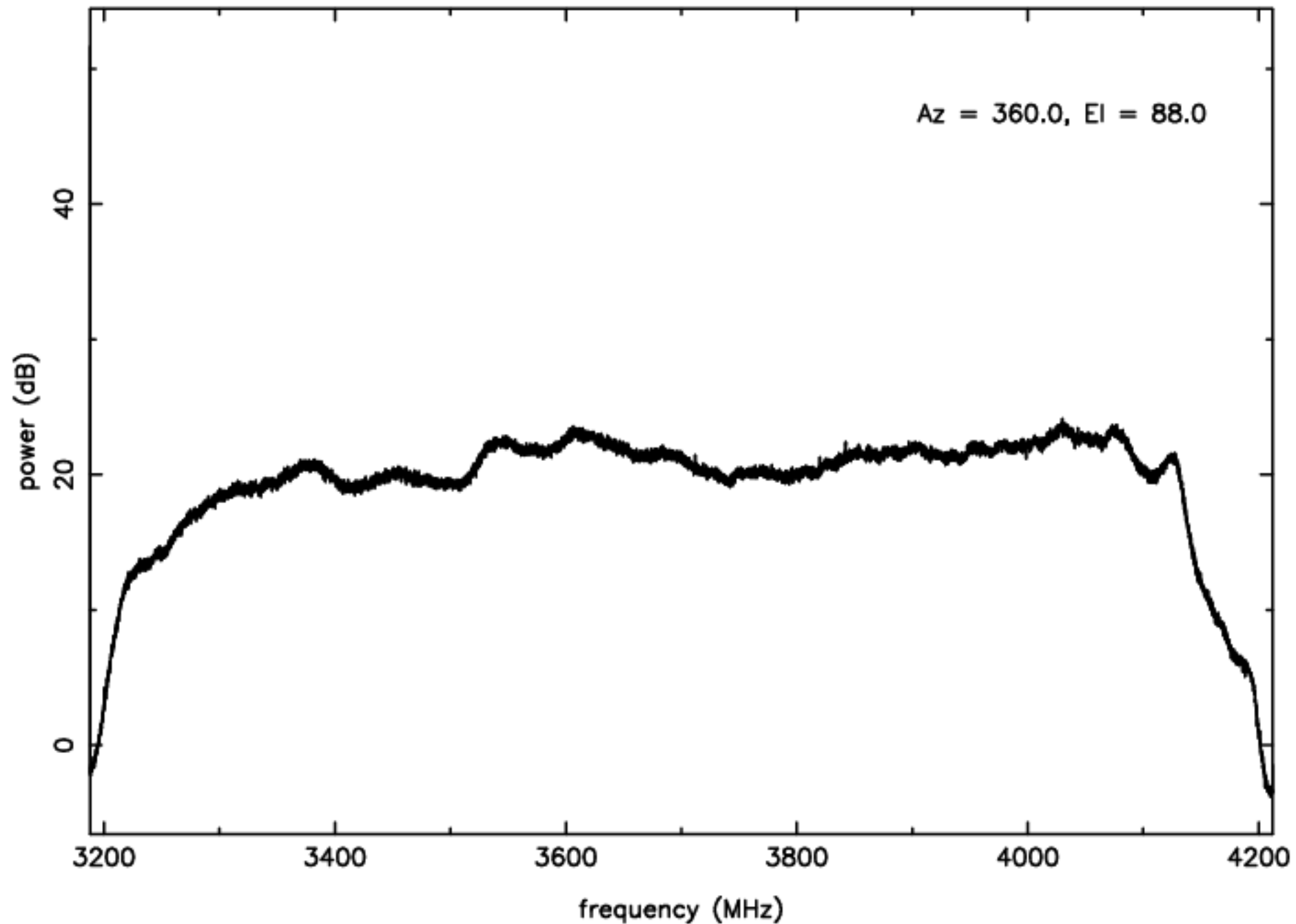
S-band RFI plot (mean power) – IF D – ea12
