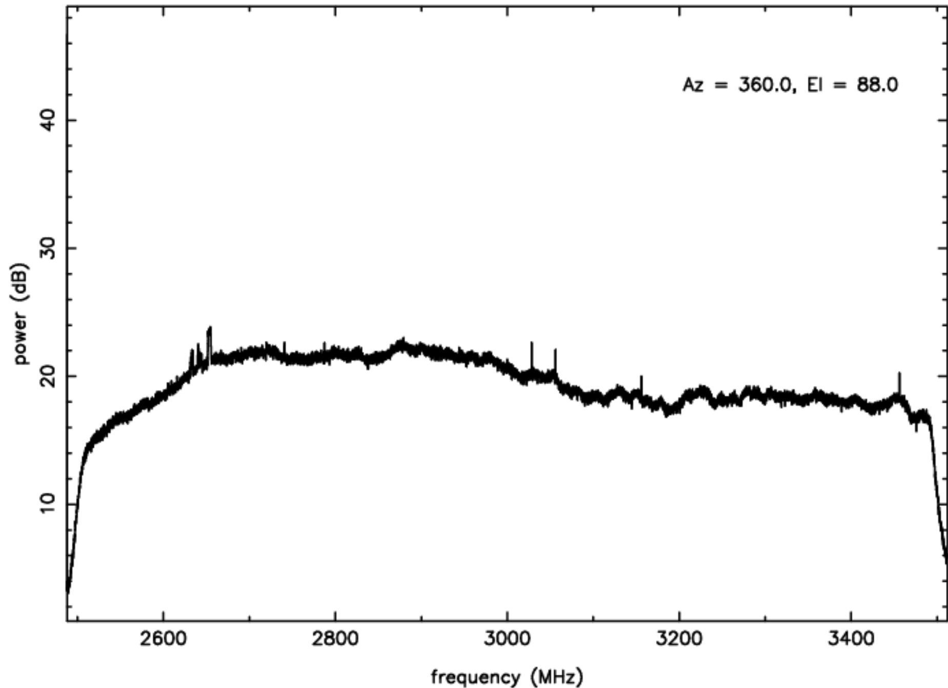
S-band RFI plot (mean power) – IF B – ea12
