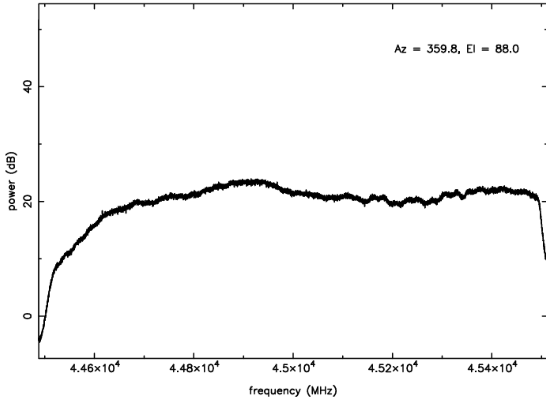
Q-band RFI plot (mean power) – IF D – ea12
