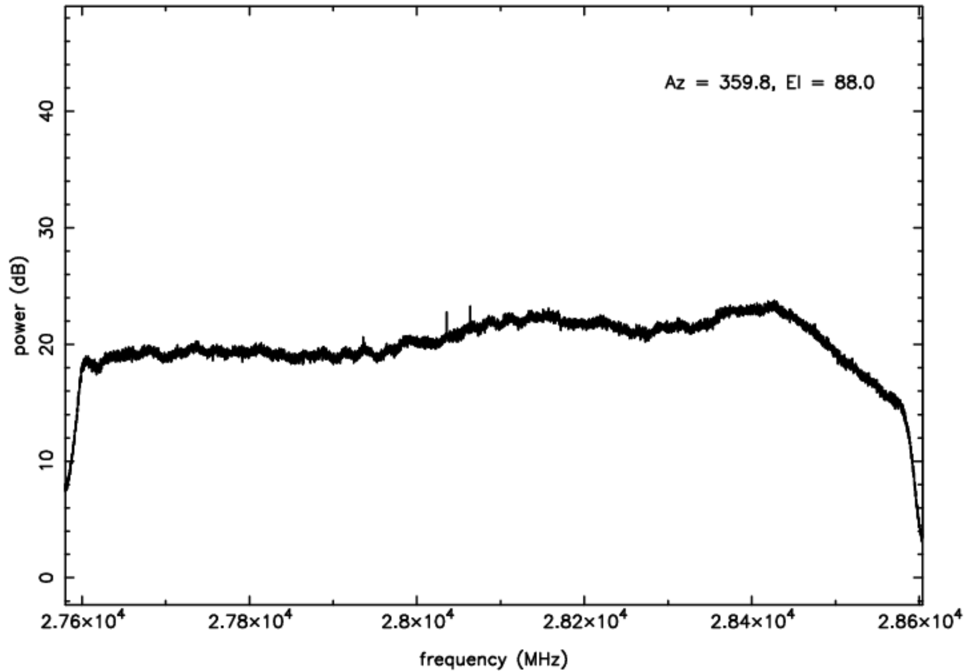
Q-band RFI plot (mean power) – IF B – ea12
