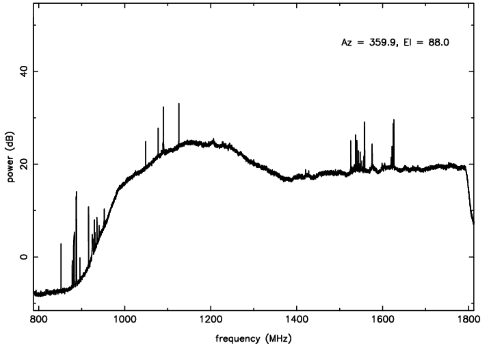
L-band RFI plot (mean power) – IF D – ea12
