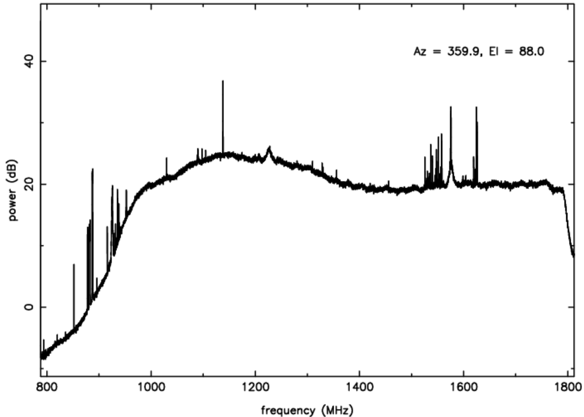
L-band RFI plot (mean power) – IF B – ea12
