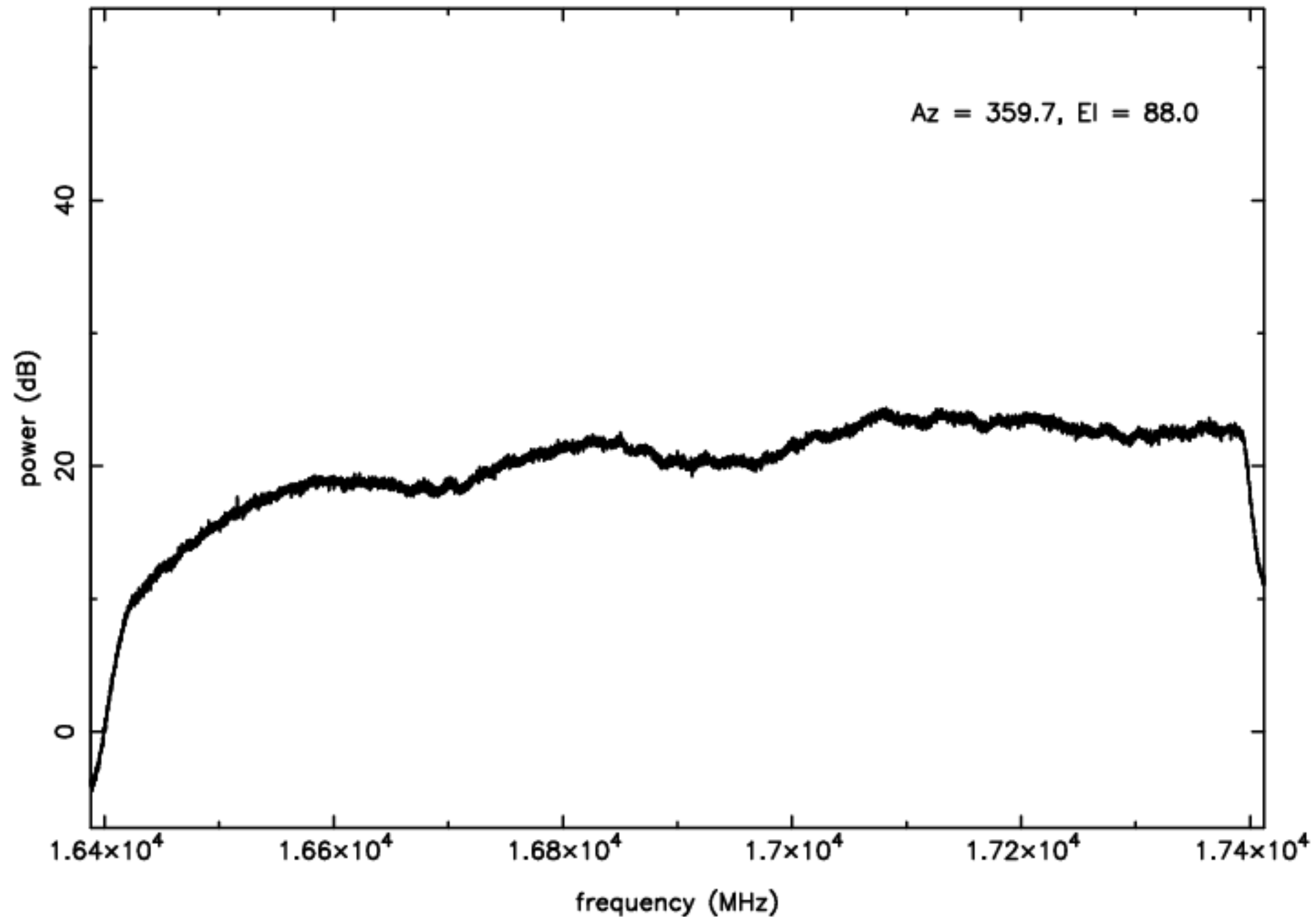
Ku-band RFI plot (mean power) - IF D - ea12
