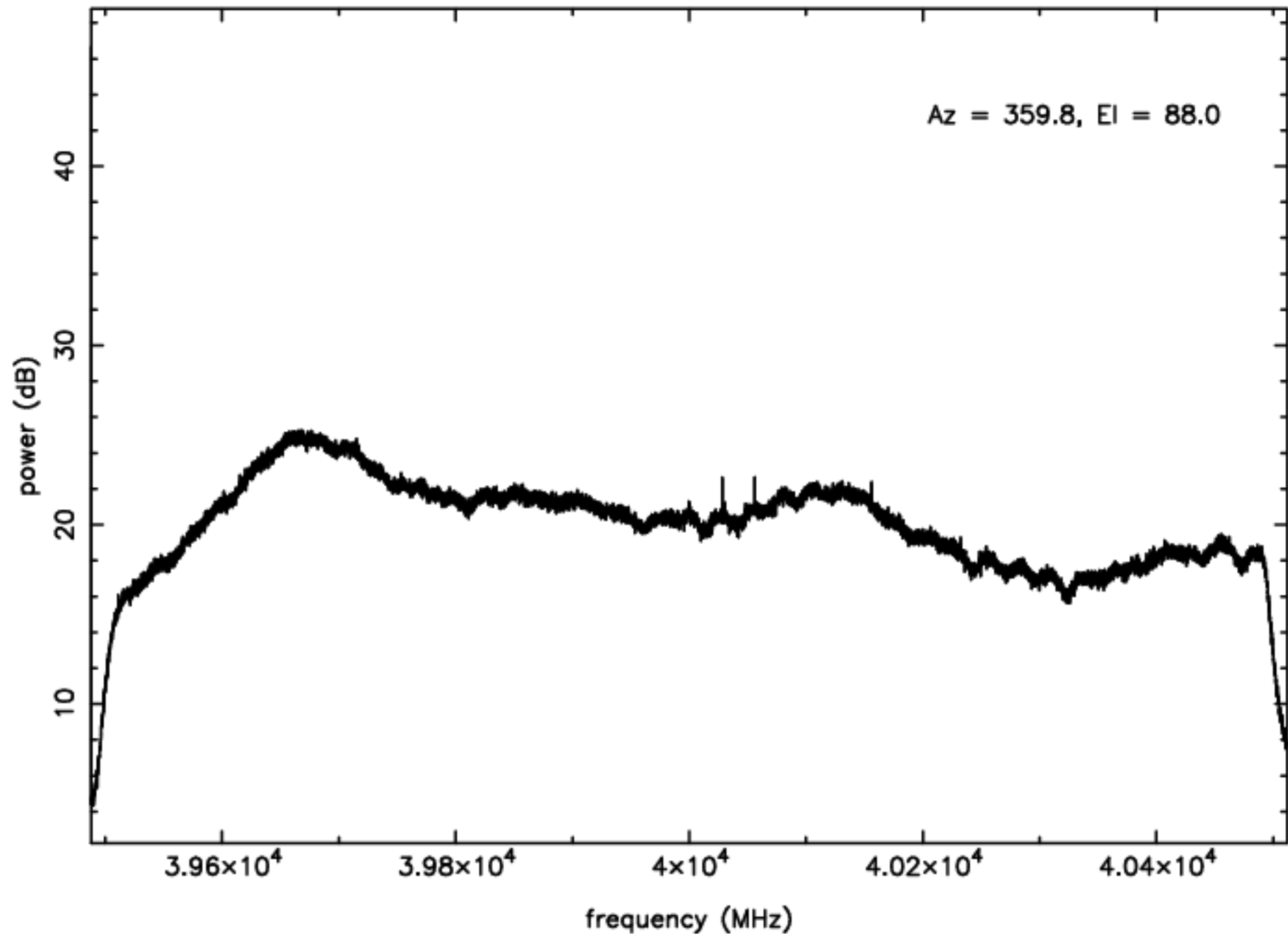
Ka-band RFI plot (mean power) – IF B – ea12
