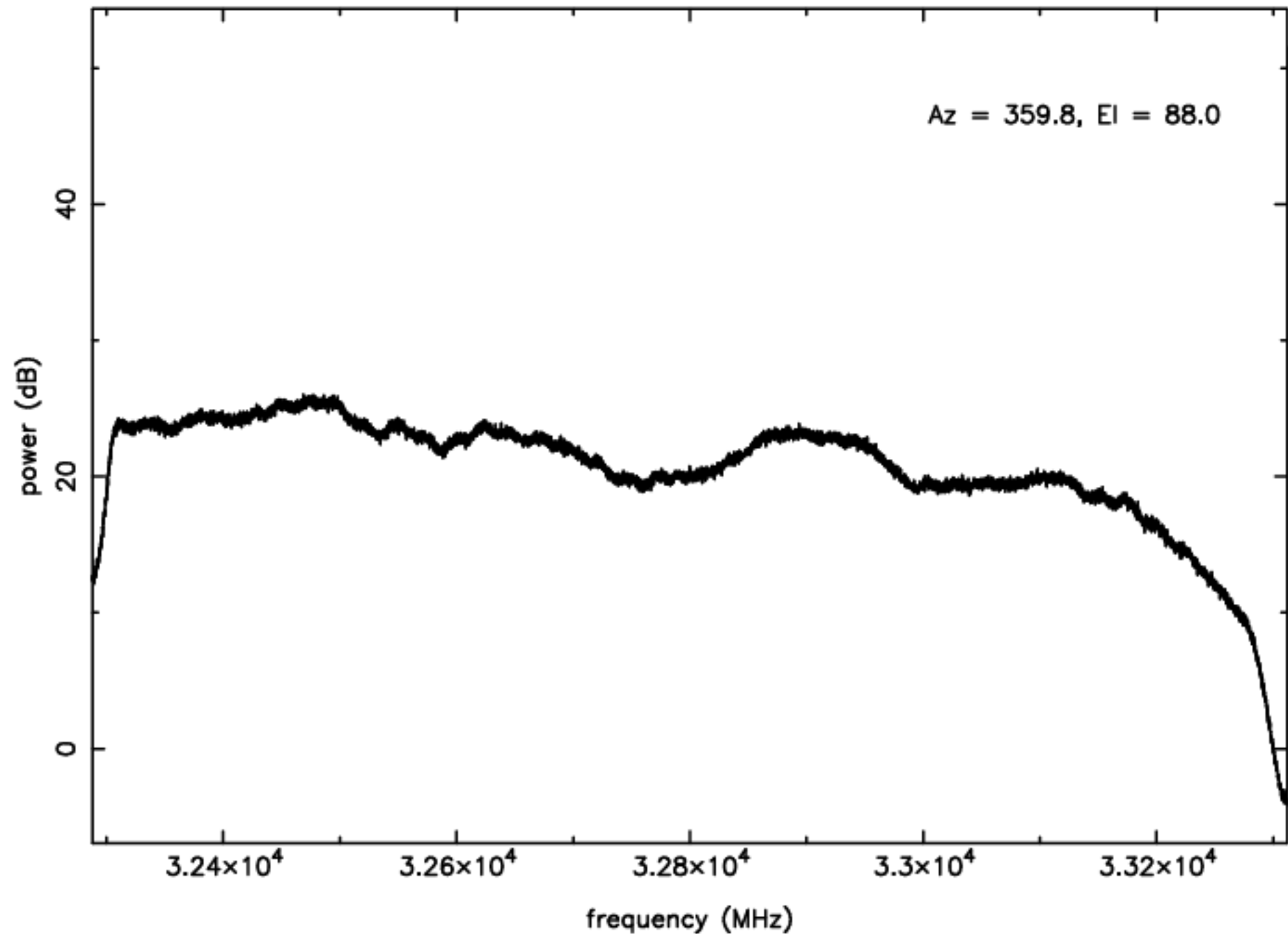
Ka-band RFI plot (mean power) – IF D – ea12
