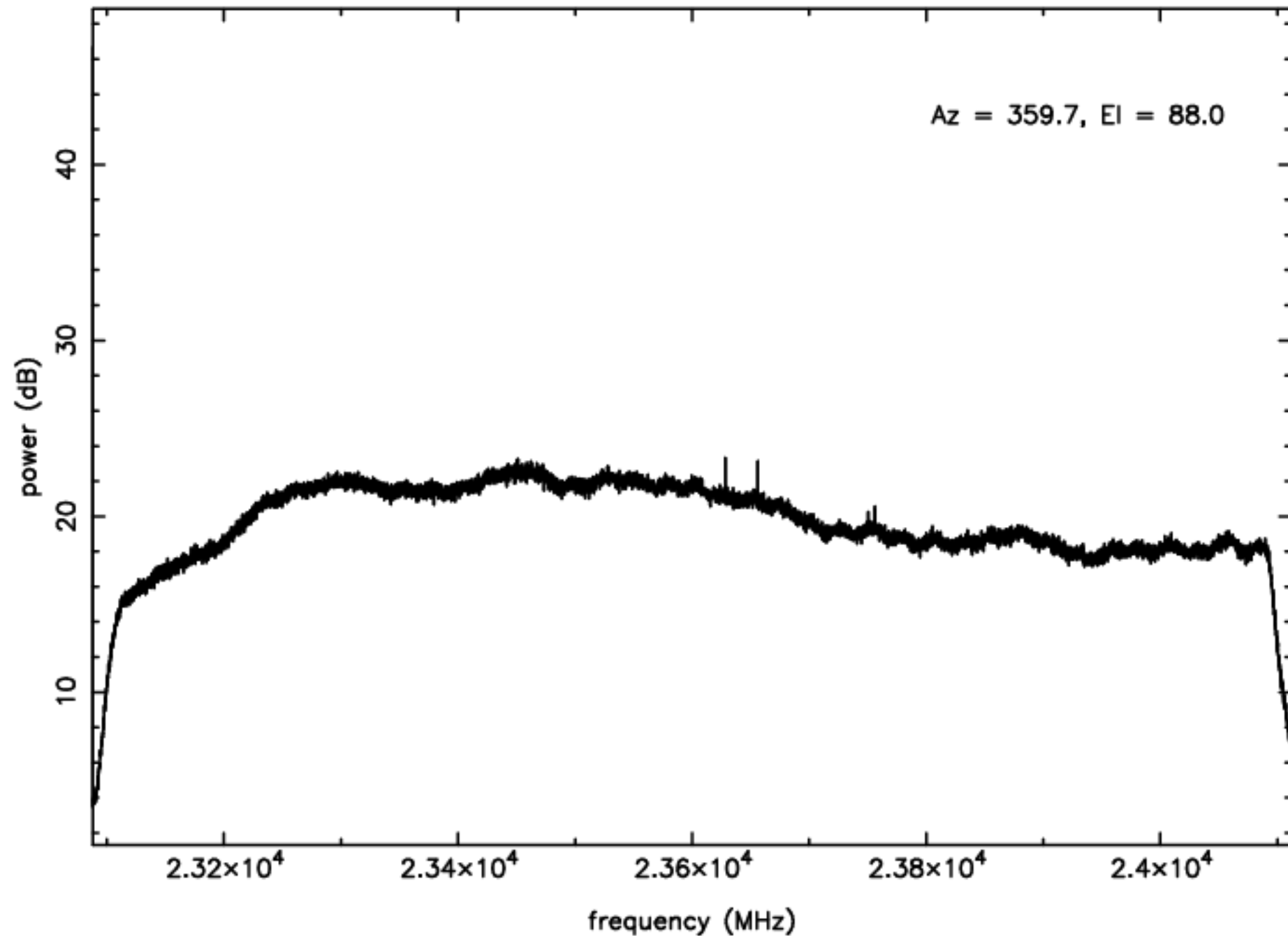
K-band RFI plot (mean power) – IF B – ea12
