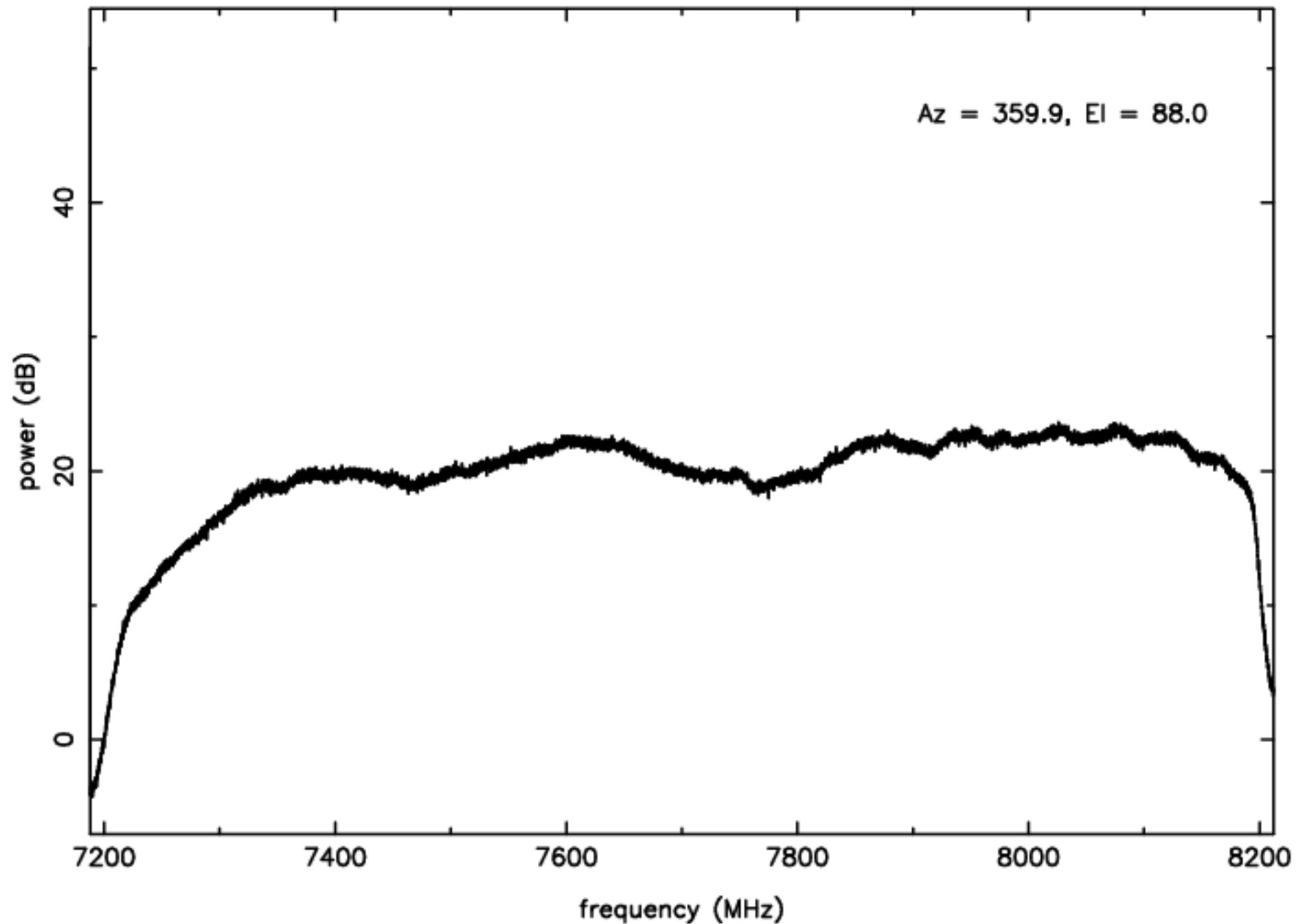
C-band RFI plot (mean power) – IF D – ea12
