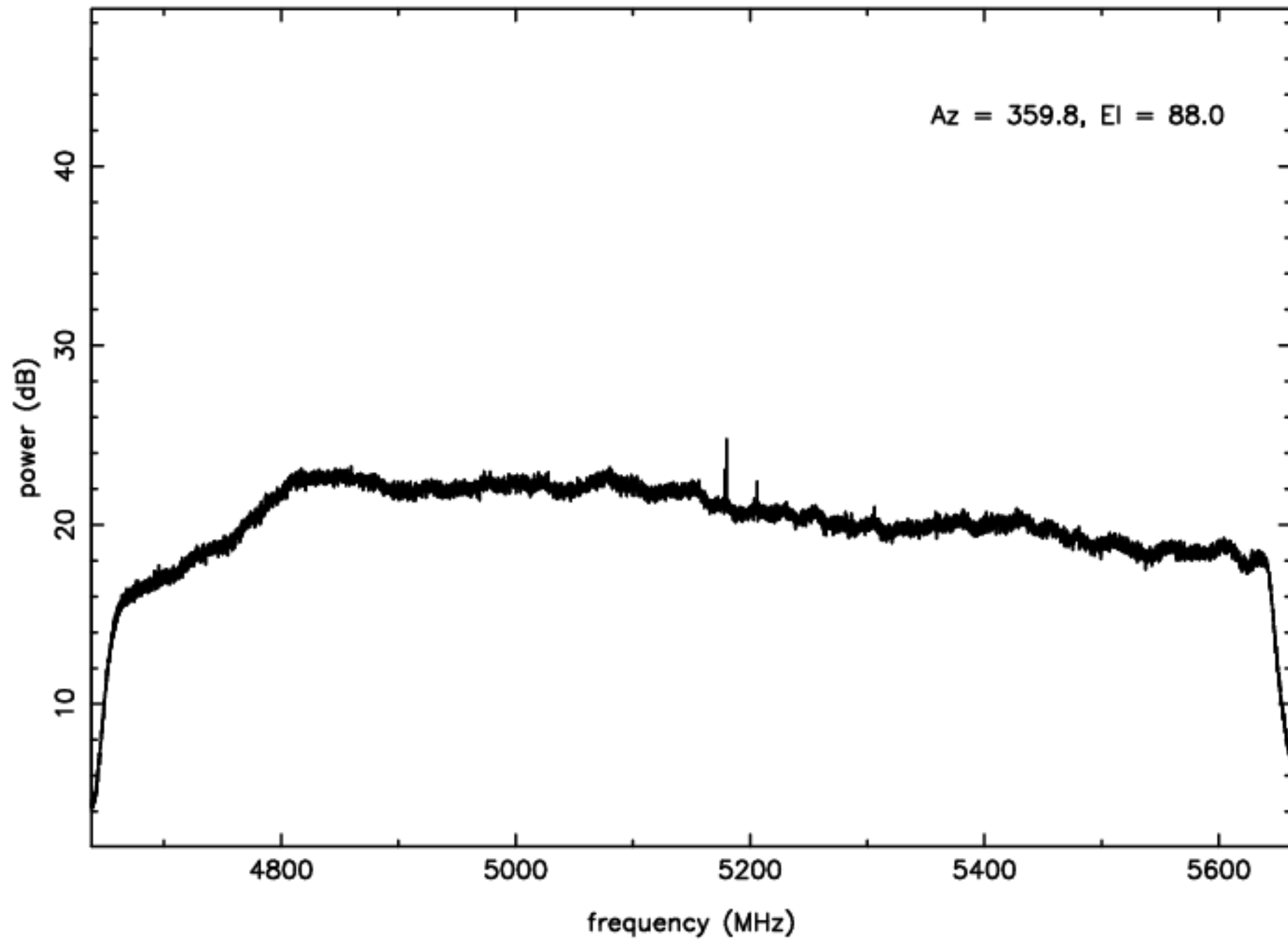
C-band RFI plot (mean power) – IF B – ea12
