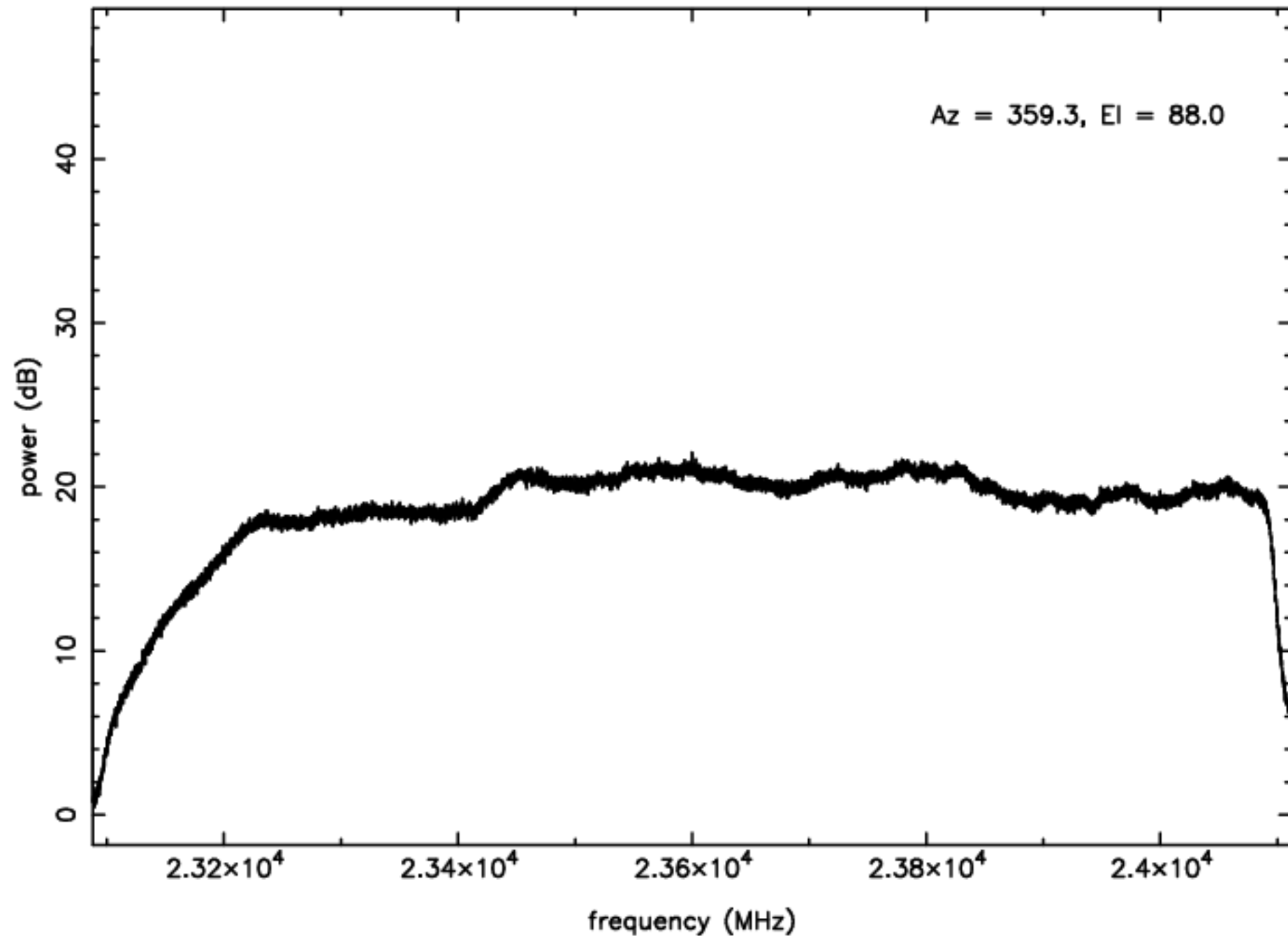
K-band RFI plot (mean power) – IF D – ea10
