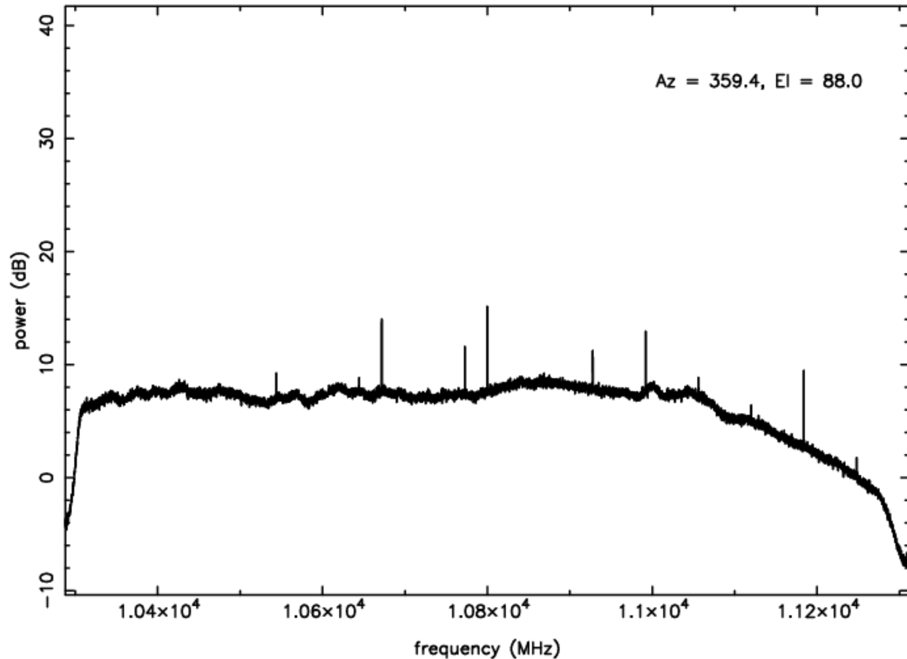
X-band RFI plot (mean power) – IF D – ea24
