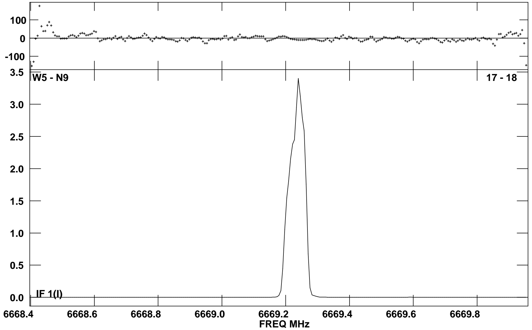
Lower frame: Kilo Ampl Jy Top frame: Phas deg Scalar averaged cross-power spectrum Baseline: EVLA:W5 (17) - EVLA:N9 (18)
