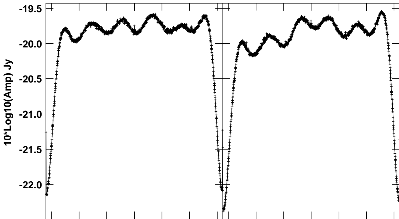
47.76 47.78 47.80 47.82 47.84 47.86 47.88 Frequency GHz IF 7(RR) IF 7(LL) Scalar averaged cross-power spectrum Several baselines averaged
