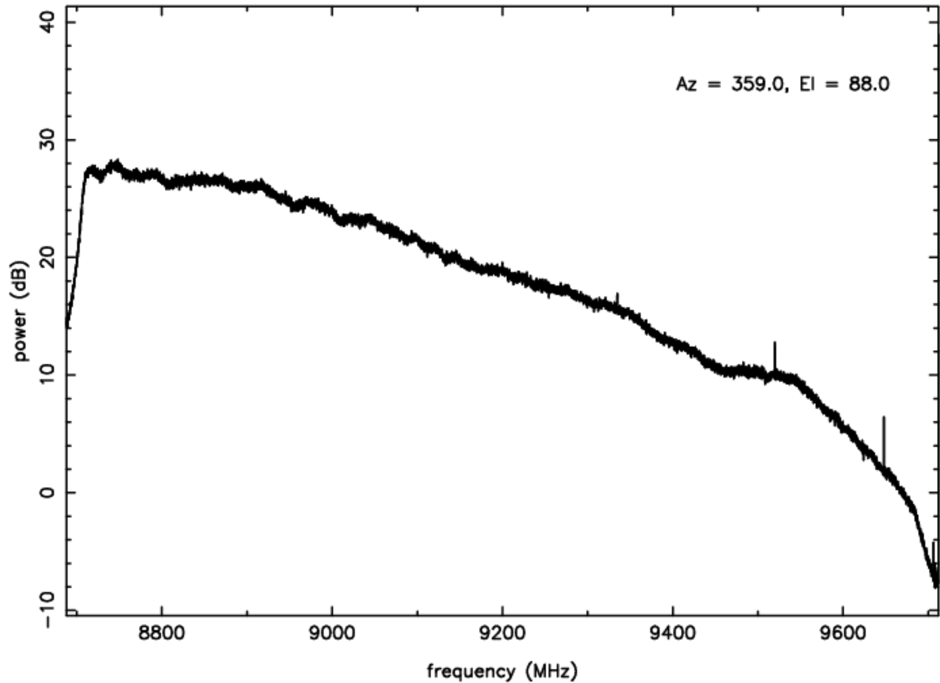
X-band RFI plot (mean power) – IF D – ea22
