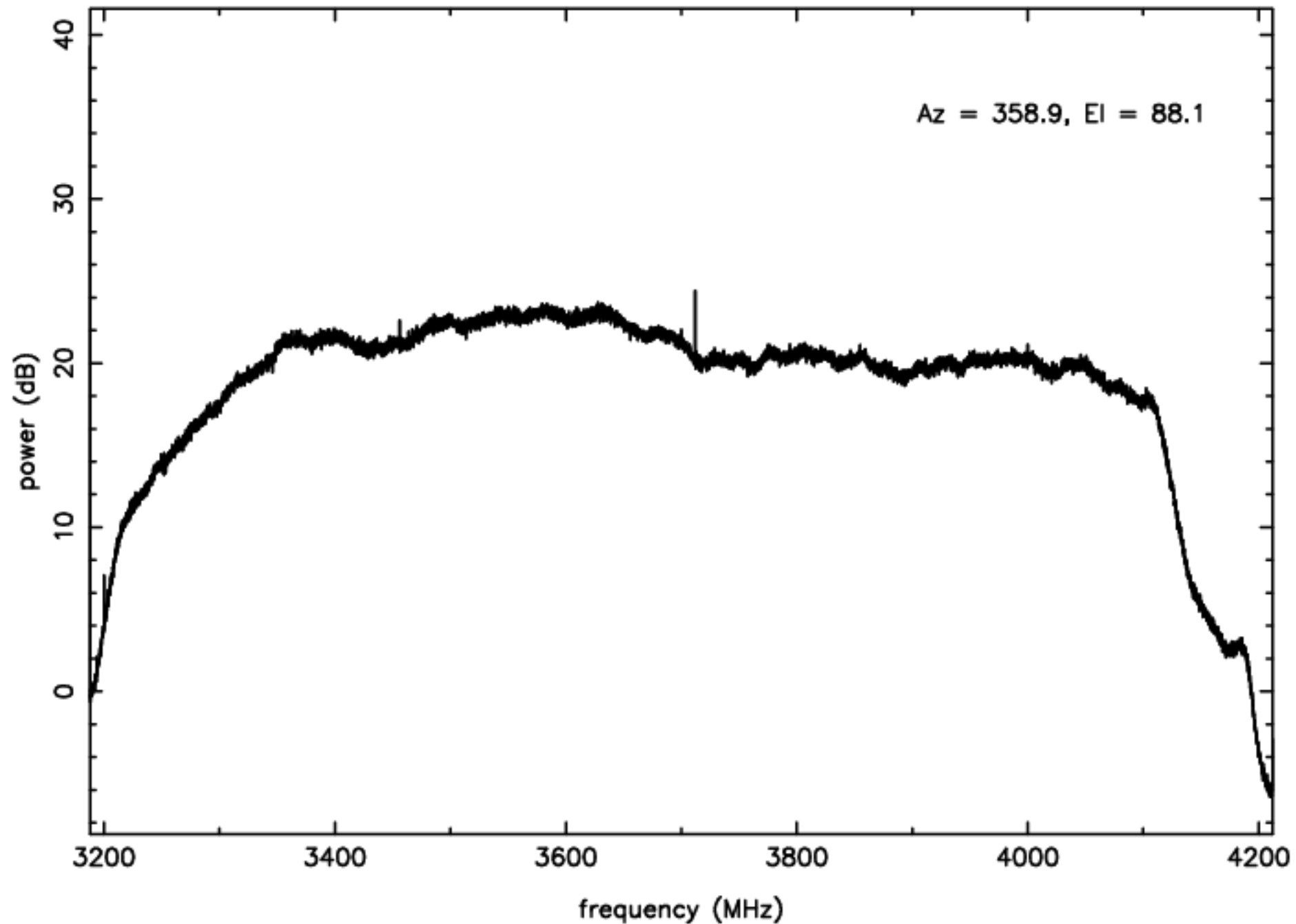
S-band RFI plot (mean power) – IF D – ea22
