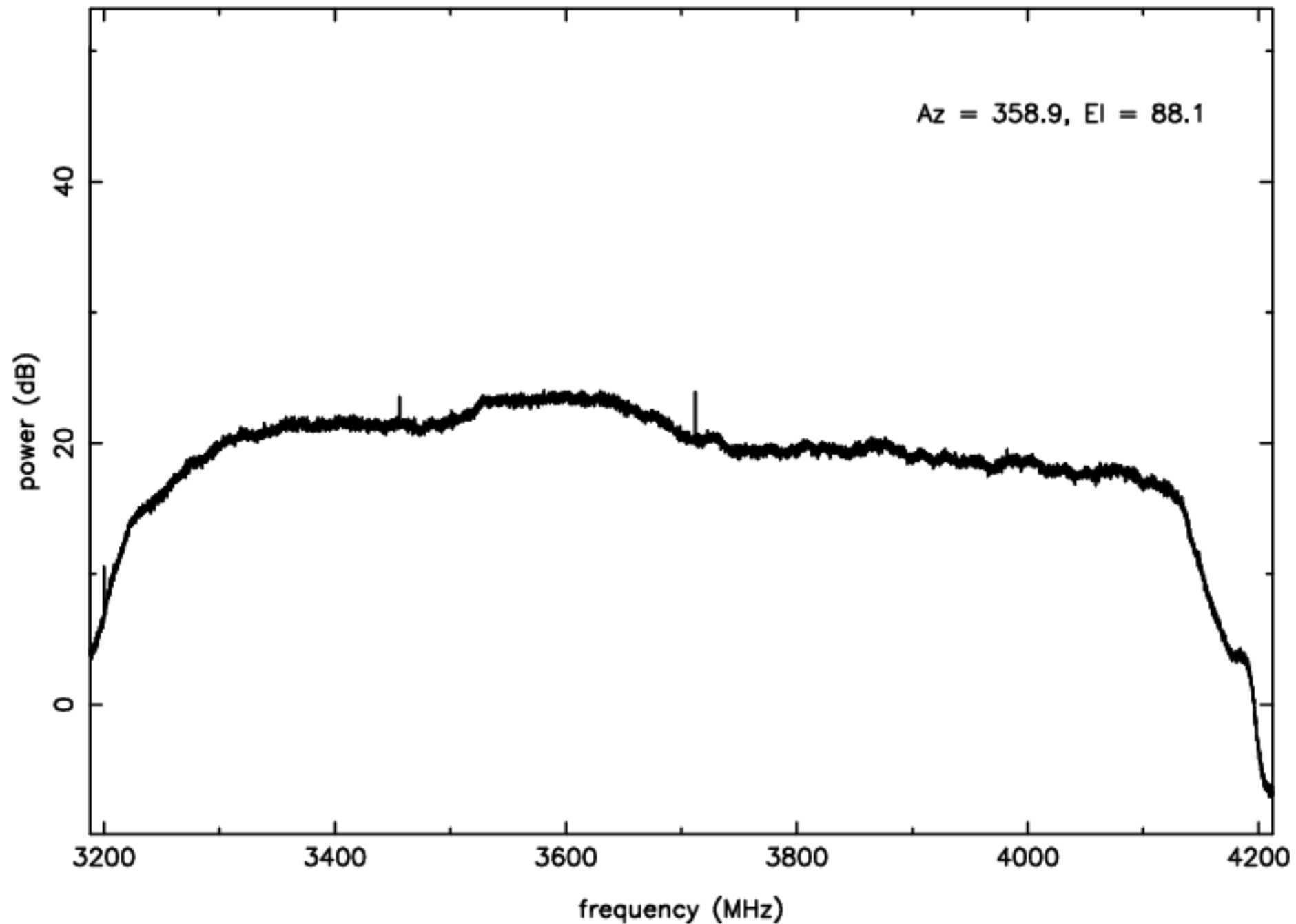
S-band RFI plot (mean power) – IF B – ea22
