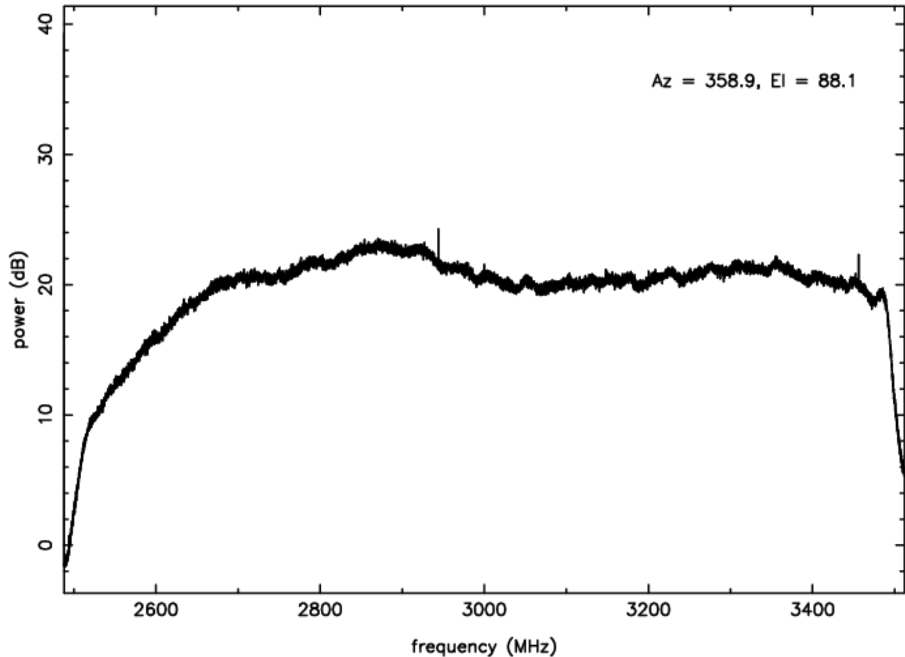
S-band RFI plot (mean power) – IF D – ea22
