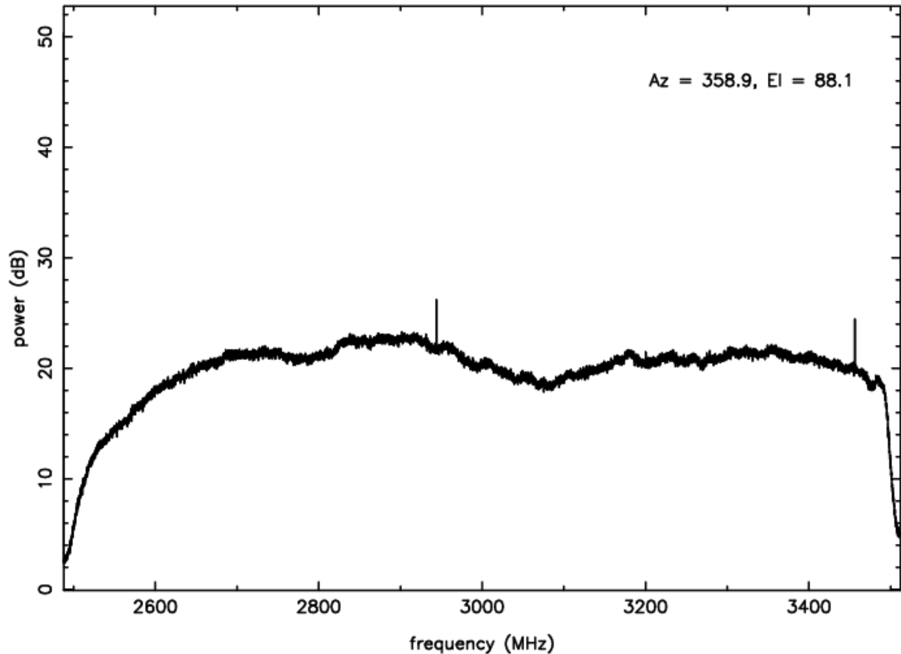
S-band RFI plot (mean power) – IF B – ea22
