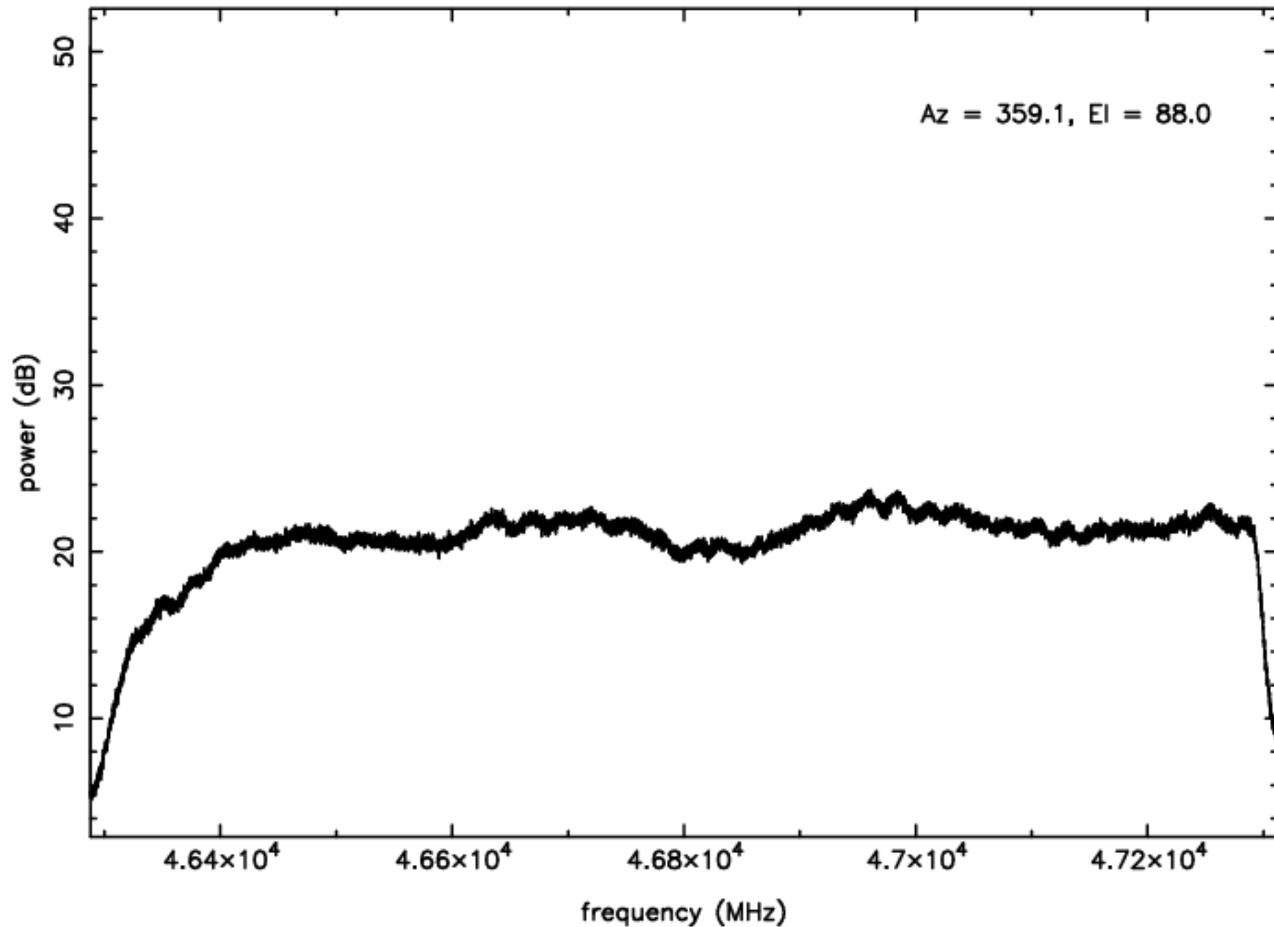
Q-band RFI plot (mean power) – IF B – ea22
