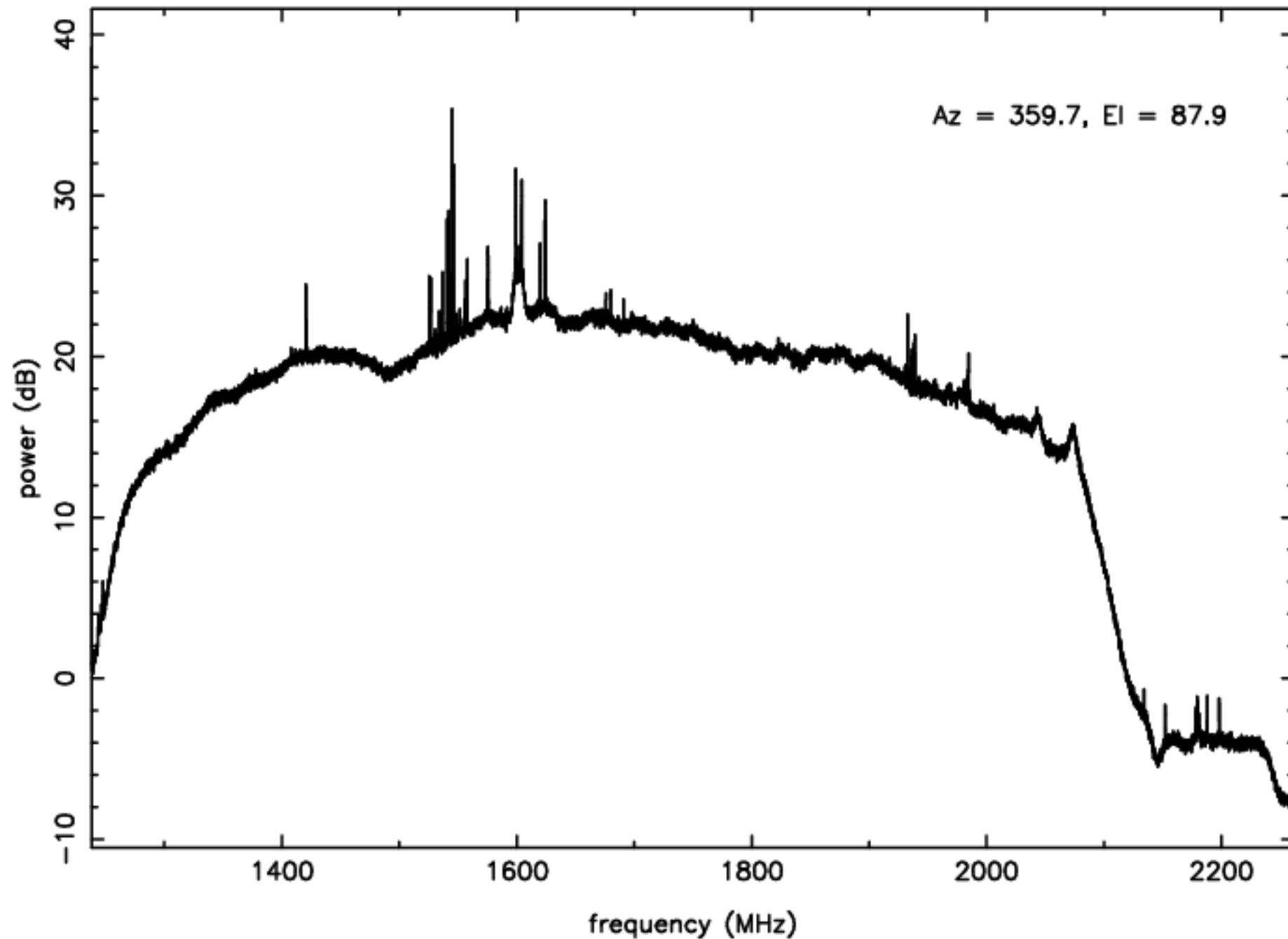
L-band RFI plot (mean power) – IF D – ea22
