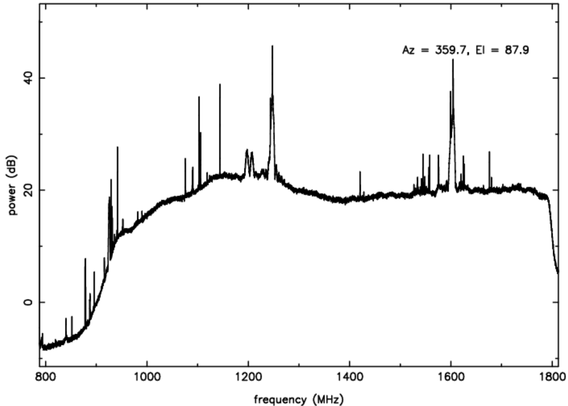
L-band RFI plot (mean power) – IF B – ea22
